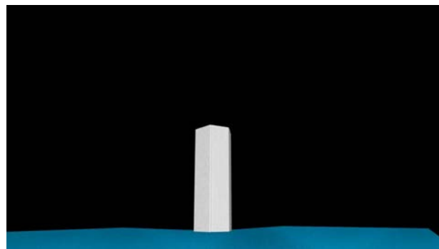
Atomistic-scale simulation
