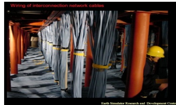
NEC Earth Simulator (640x640 crossbar)
