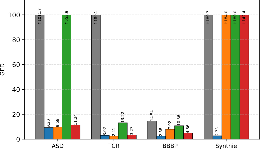
GED (lower is better)
