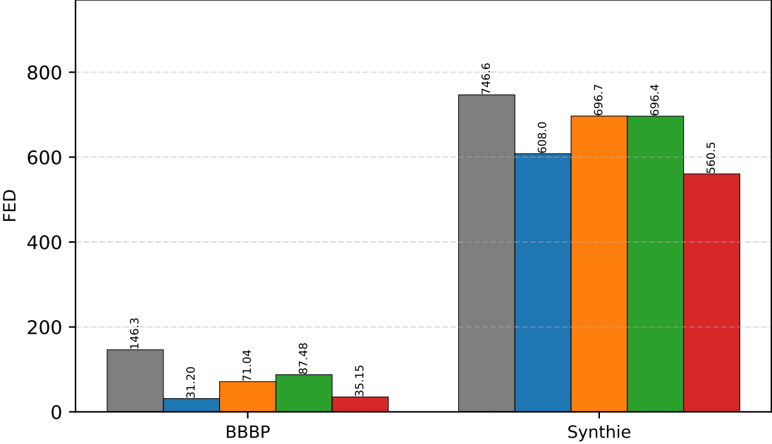
FED (lower is better)
