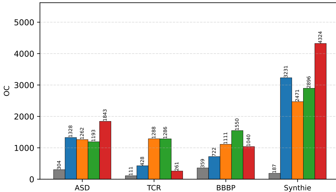
Oracle Calls (lower is better)
