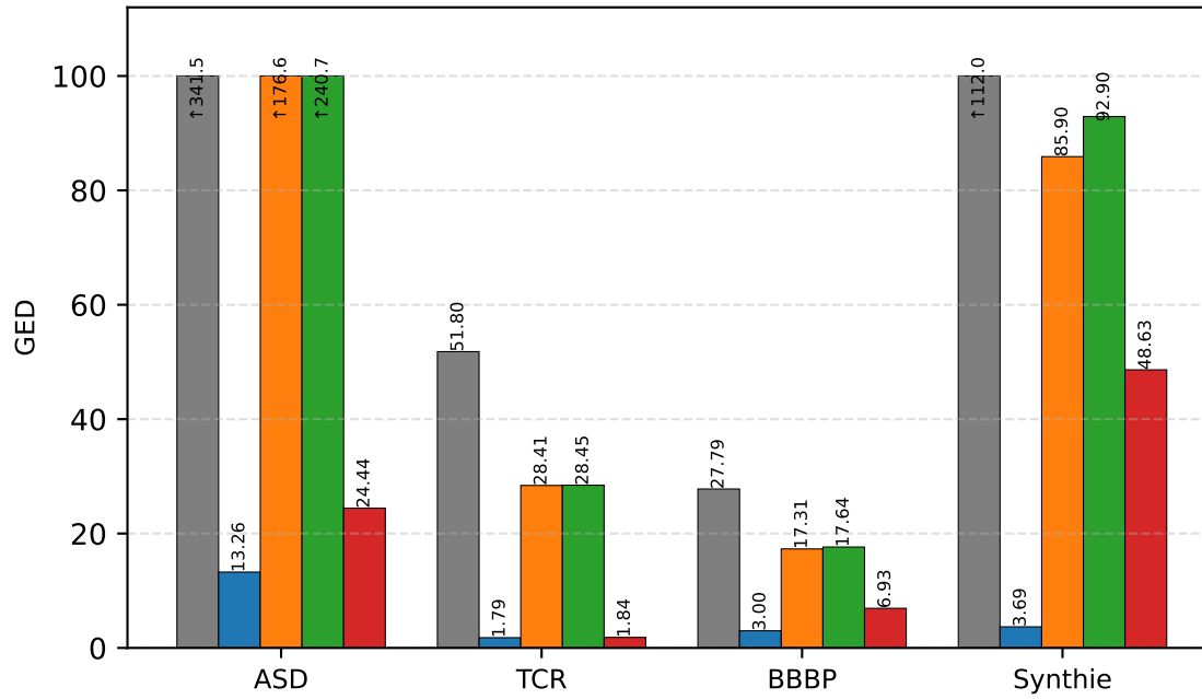
GED (lower is better)
