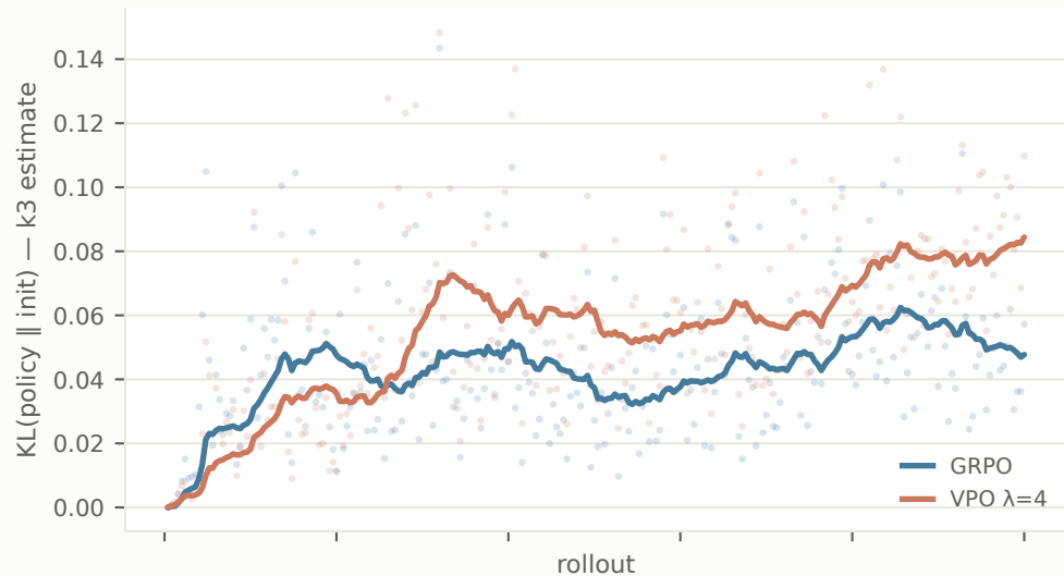
Llama-3.1-8B Instruct → RL
