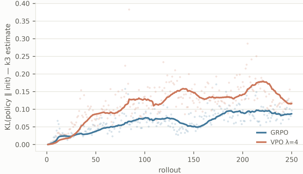
Llama-3.1-8B Instruct → RL
