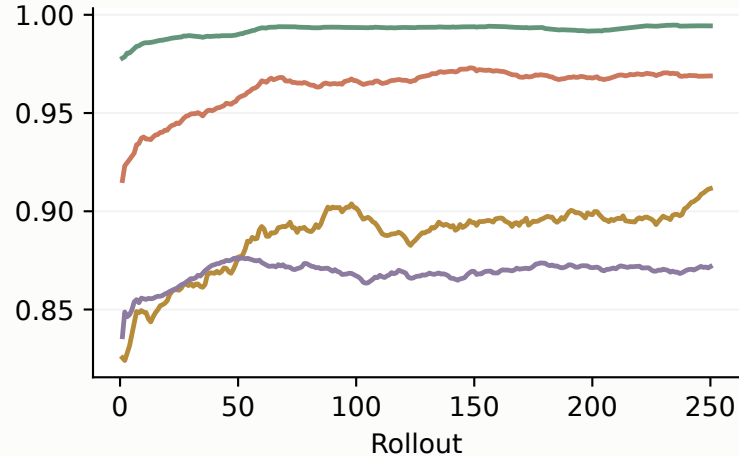
Credit ESS ratio
