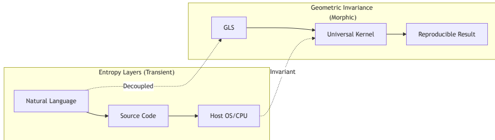
Figure 1: Principle of Decoupling Intelligence from Environmental Entropy
