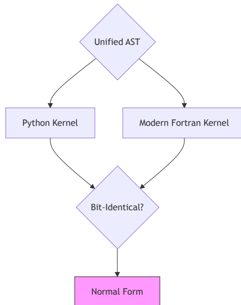
Figure 7: Deterministic Kernel Parity.** This visualization shows a single universal logic form processed by independent execution kernels (Python and Fortran), both converging on a bit-identical Normal Form
