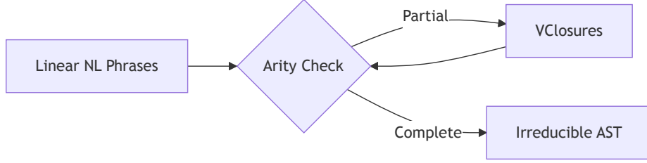
Figure 3: Recursive Folding Logic.** This visualization demonstrates how primitives are recursively composed into a universal logic form by strictly validating arity constraints \alpha(P) against incoming arguments
