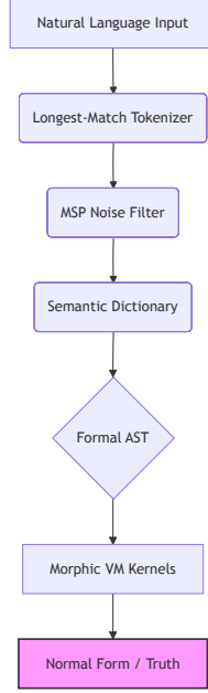
Figure 1: Global Architecture of Morphic Inner World.** This diagram illustrates the deterministic progression from ambiguous natural language to a verified normal form through structure-preserving stages
