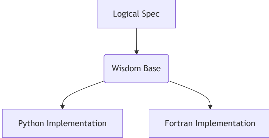
Figure 2: Substrate Independence Layer.** The Wisdom Base functions as a cognitive registry, decoupling the universal logic (AST) from platform-specific execution kernels to ensure implementation invariance
