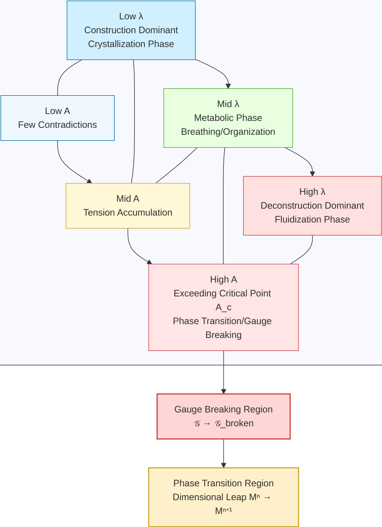
Phase Diagram: \lambda – A Plane
