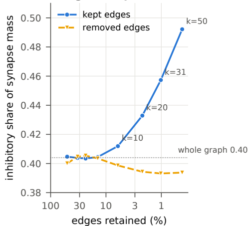
a sign of kept vs removed mass
