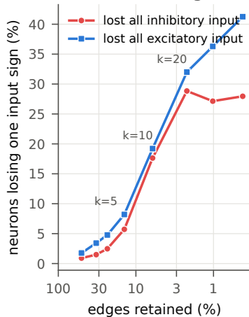
b neurons losing one input sign
