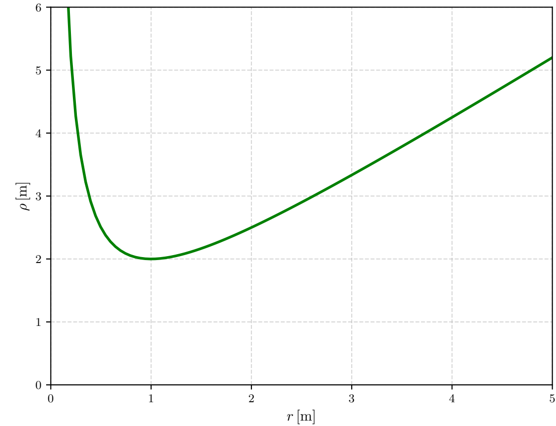
Curvature Radius vs. Helix Radius
