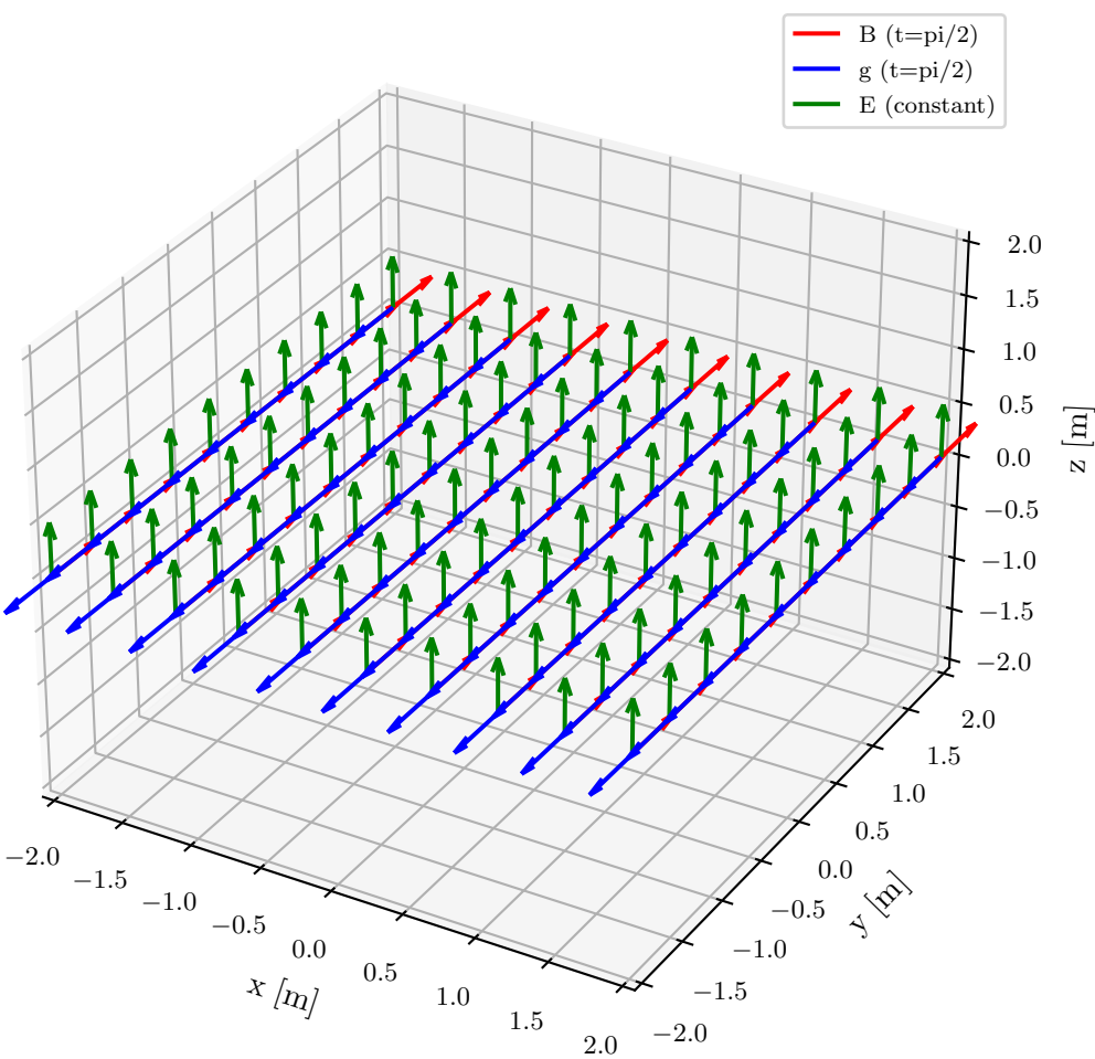
3D Field Vectors Visualization
