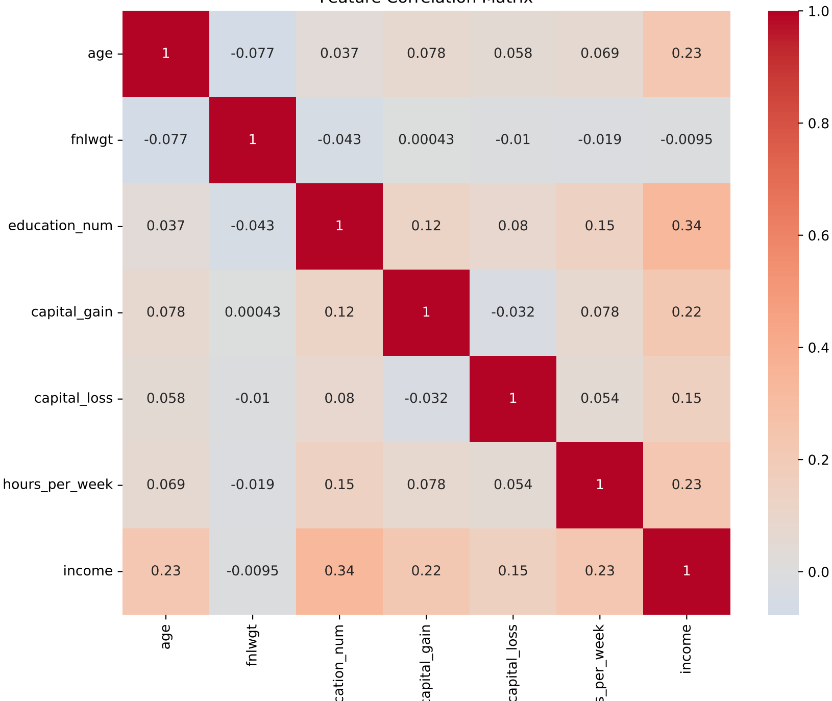
Feature Correlation Matrix
