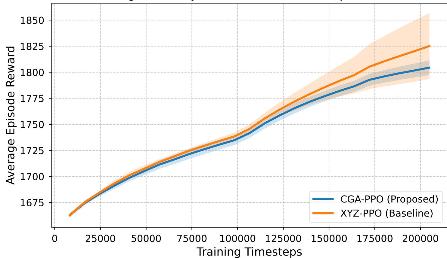
Convergence Analysis: CGA vs. Euclidean Representation
