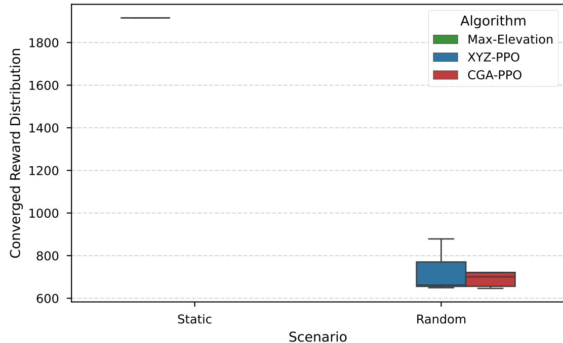
Performance Stability (Final 10% Steps)
