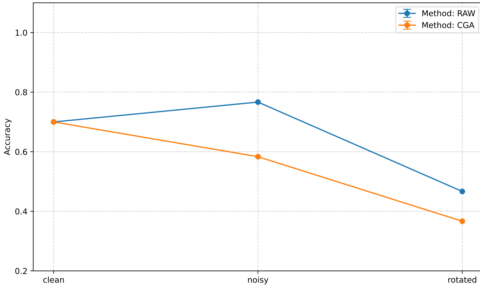
Test Accuracy Comparison: CGA-VQM vs Raw-VQC
