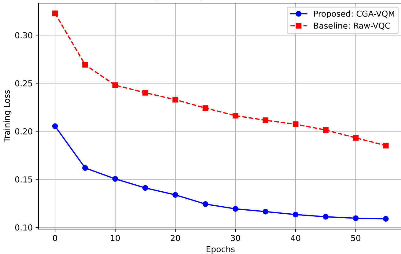
Learning Convergence (Rotated Scenario)
