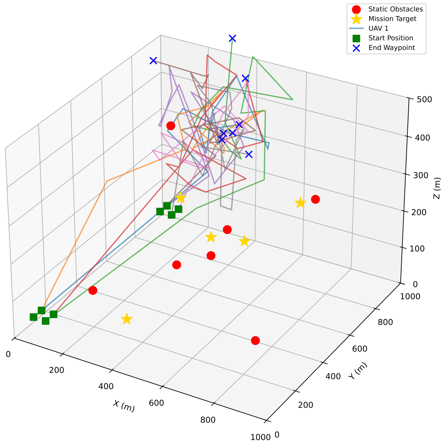
Figure 2: C-DPSO Optimized Paths - Scenario_2_CDP
