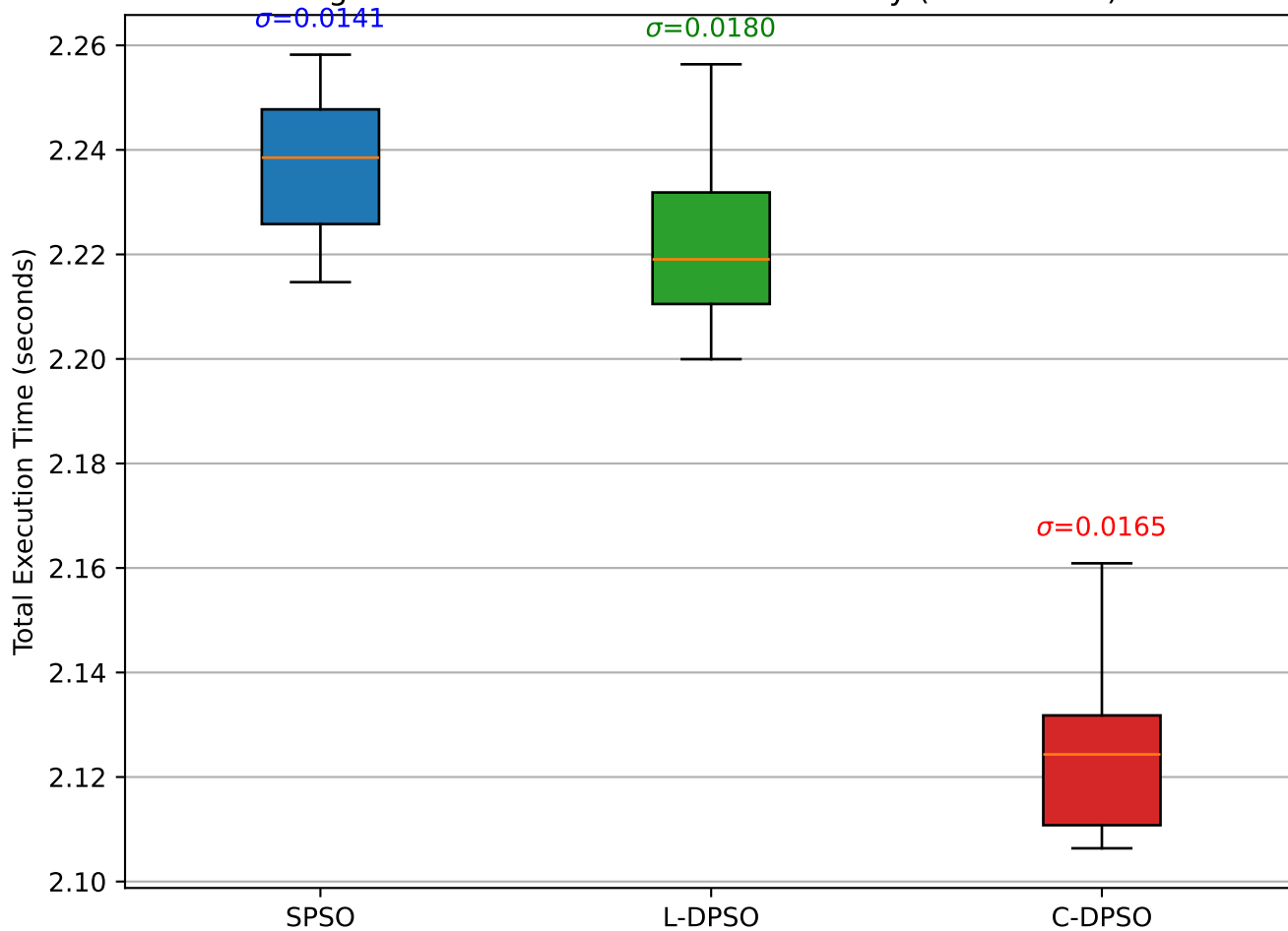
Figure 3: Execution Time Predictability (N=10 Runs)
