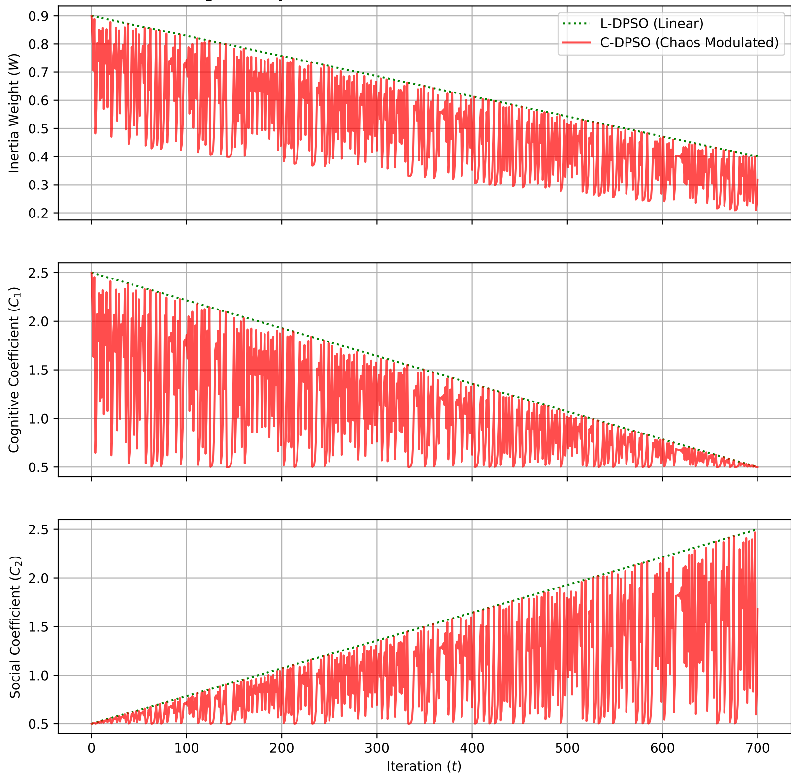
Figure 4: Dynamic Parameter Modulation (Chaos vs Linear)
