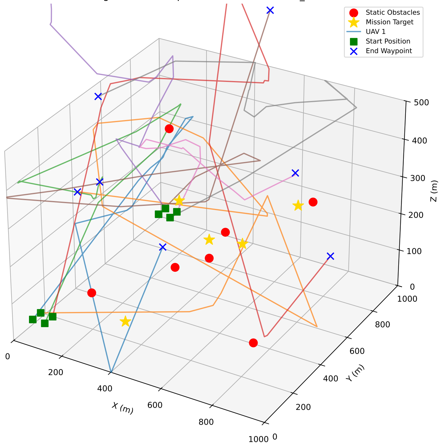
Figure 2: SPSO Optimized Paths - Scenario_2
