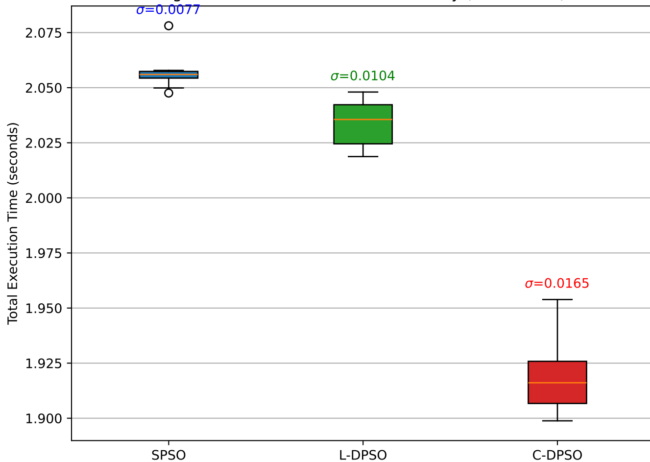
Figure 3: Execution Time Predictability (N=10 Runs)
