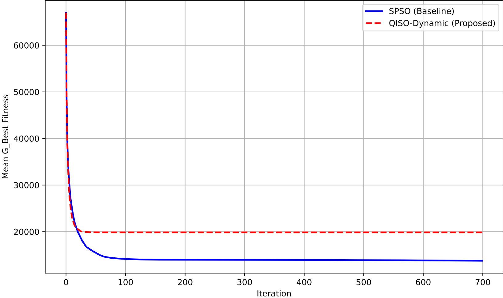
Mean Convergence Analysis (N=10) - Scenario_2_Comparison
