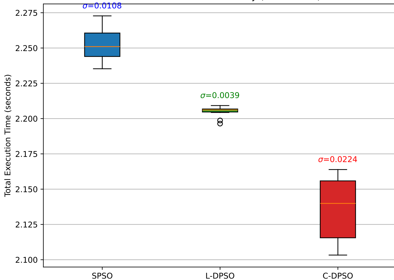
Execution Time Predictability (N=10 Runs)
