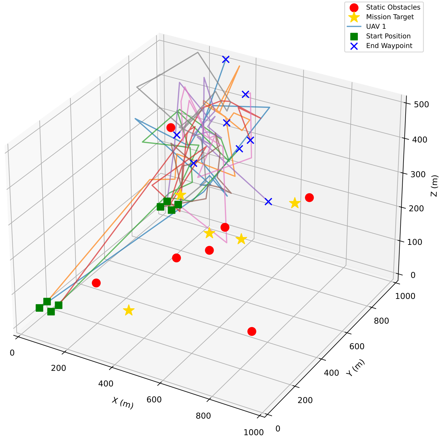
C-DPSO Optimized Paths - Scenario_2_CDP
