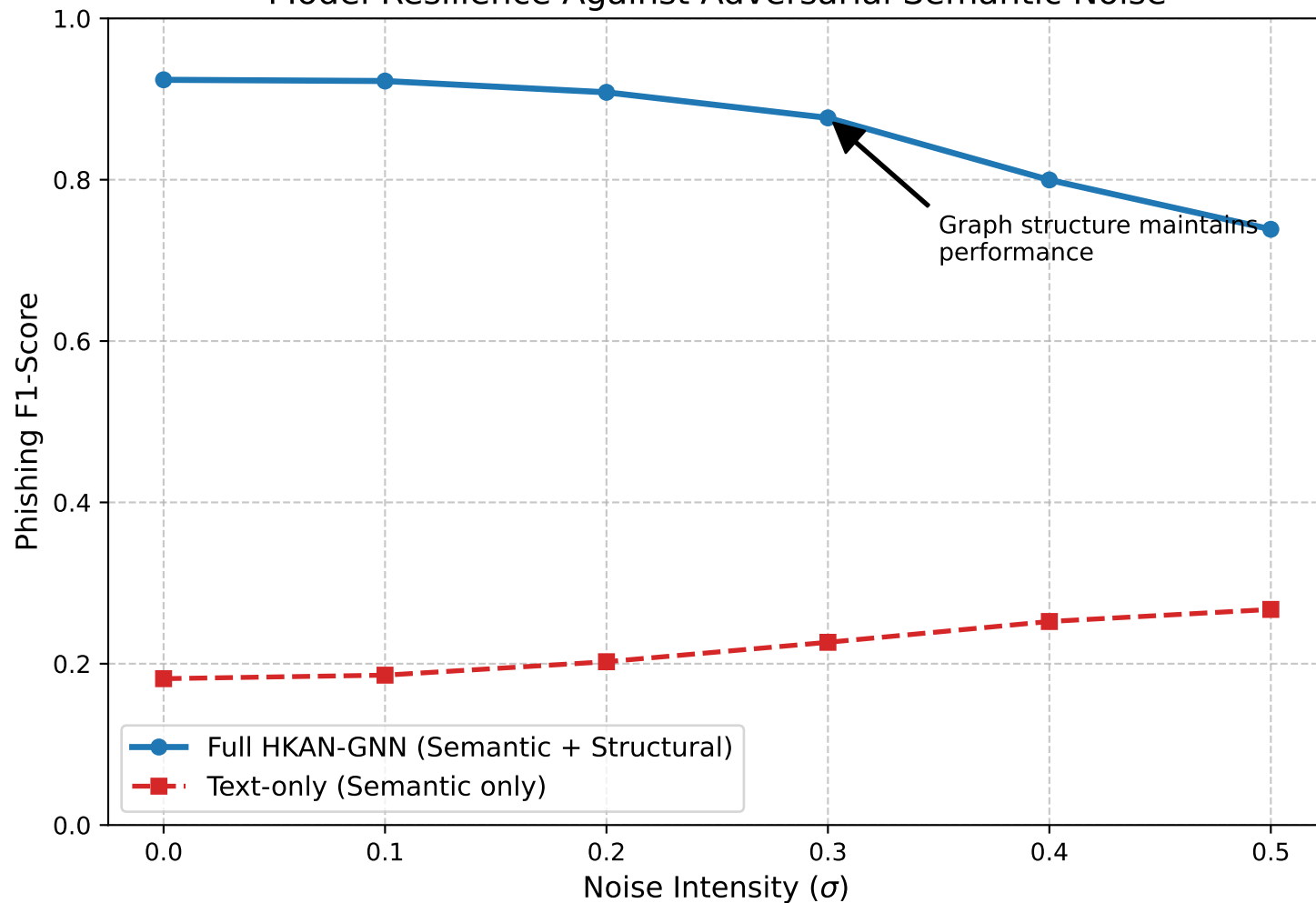
Model Resilience Against Adversarial Semantic Noise
