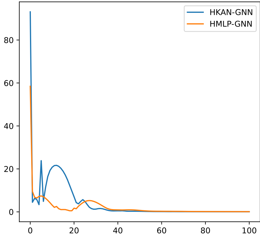
Training Loss
