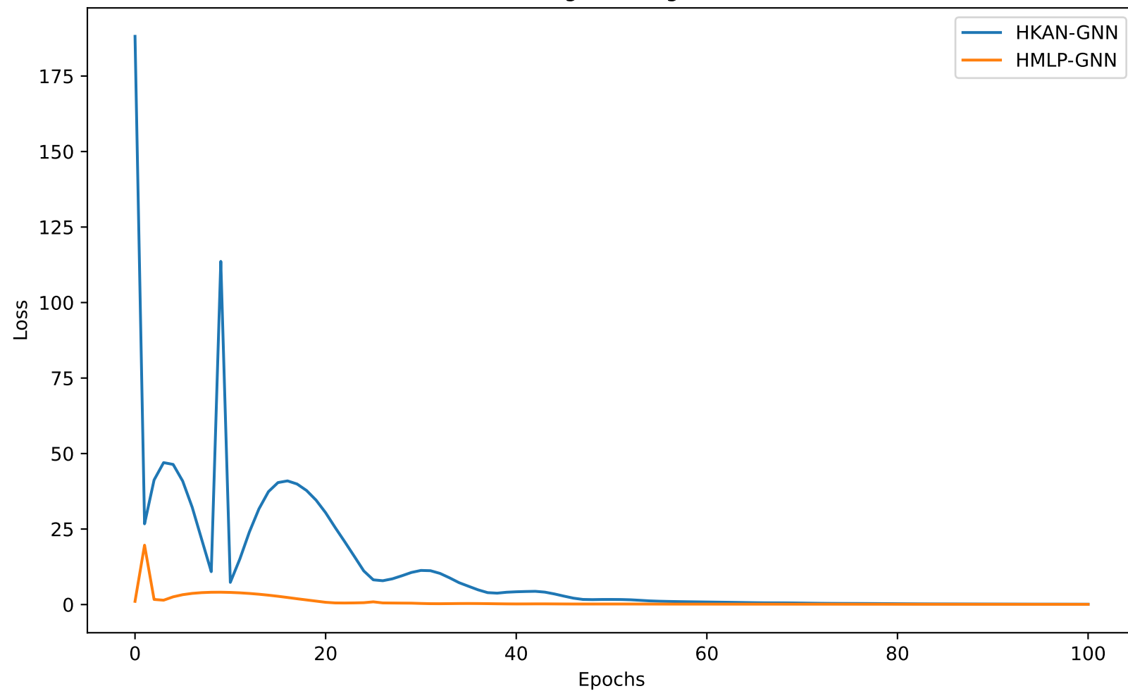
Training Convergence
