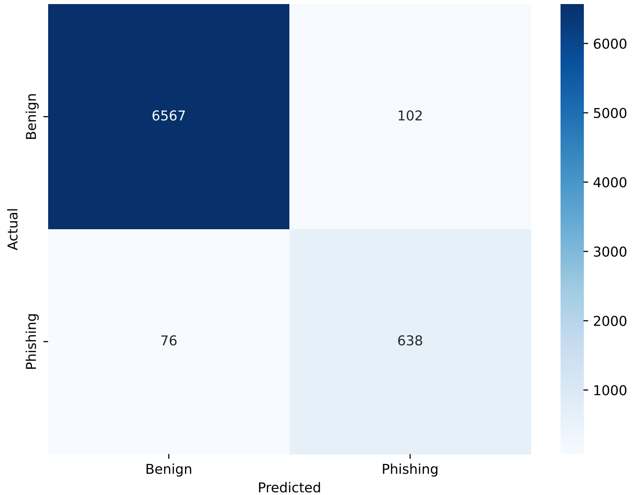
Final Confusion Matrix (Test Set)
