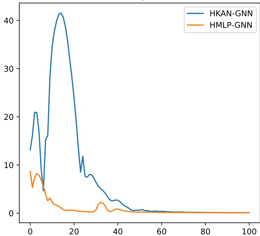
Training Loss
