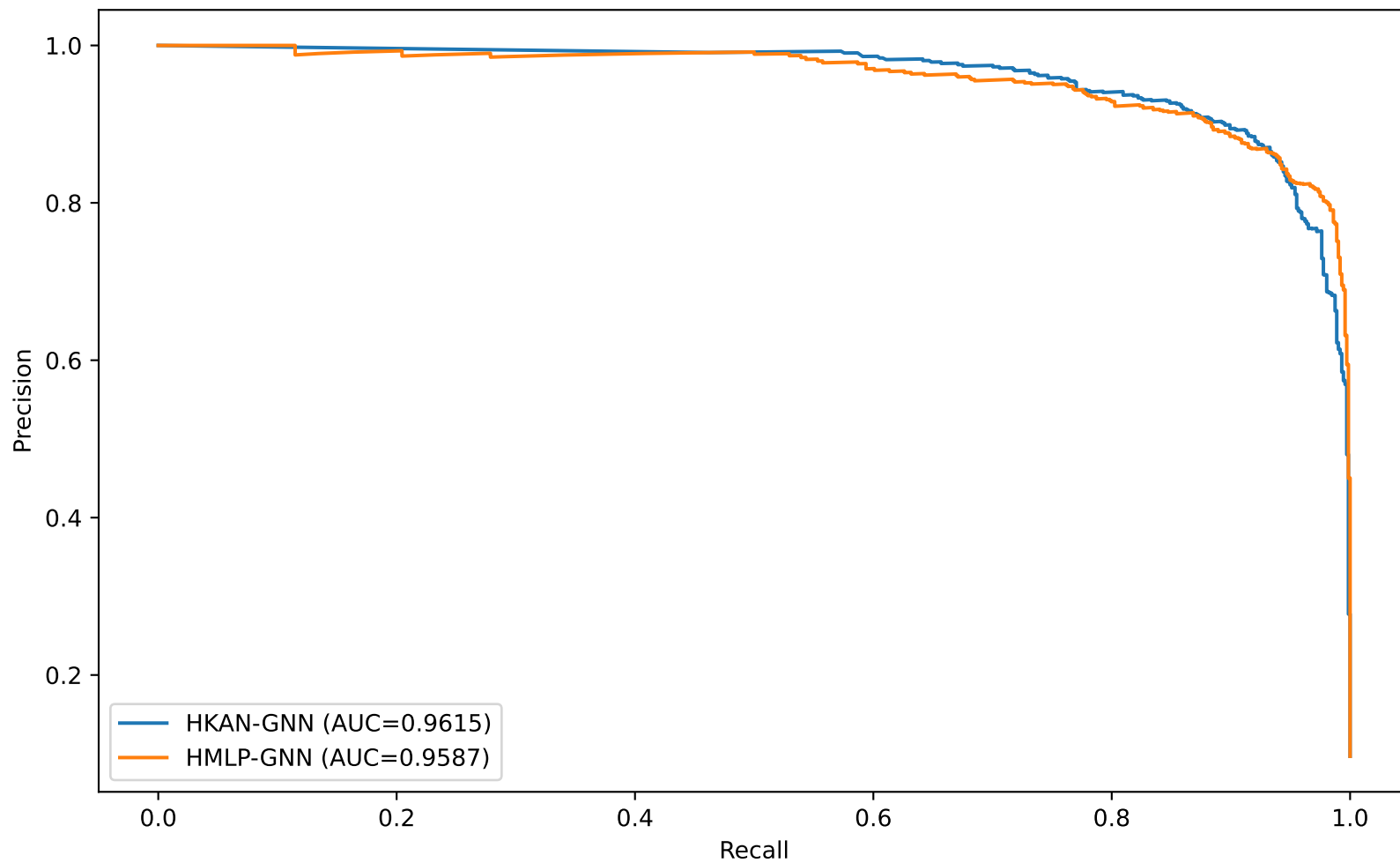
Precision-Recall Curves
