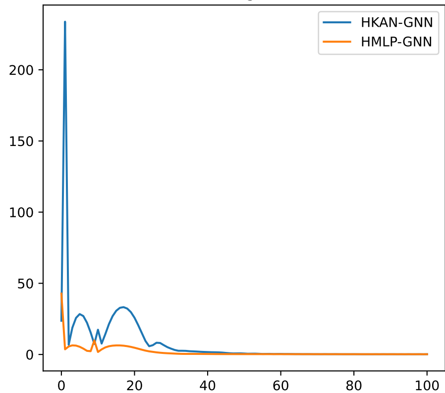
Training Loss
