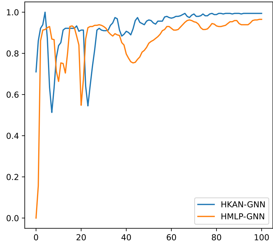
Phishing Recall (Validation)
