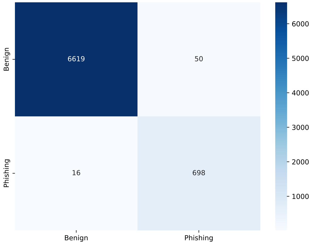
Confusion Matrix - HKAN-GNN
