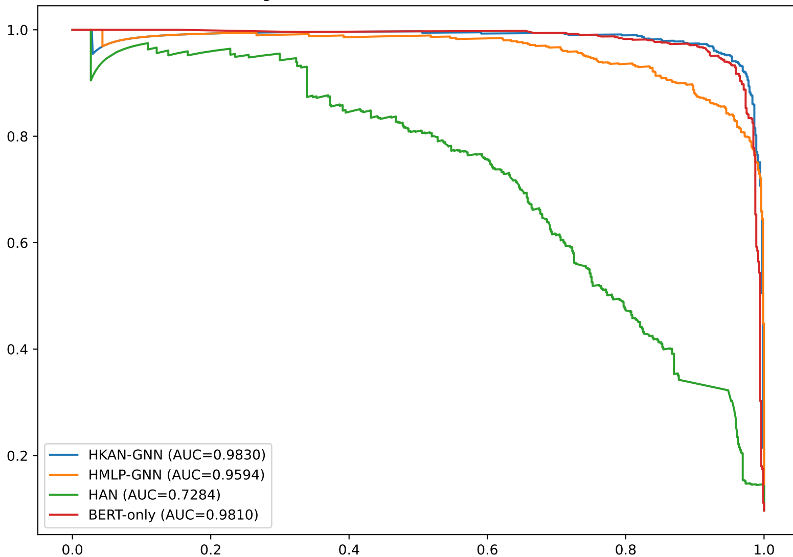
Figure 3: PR-Curves (Extended Baselines)
