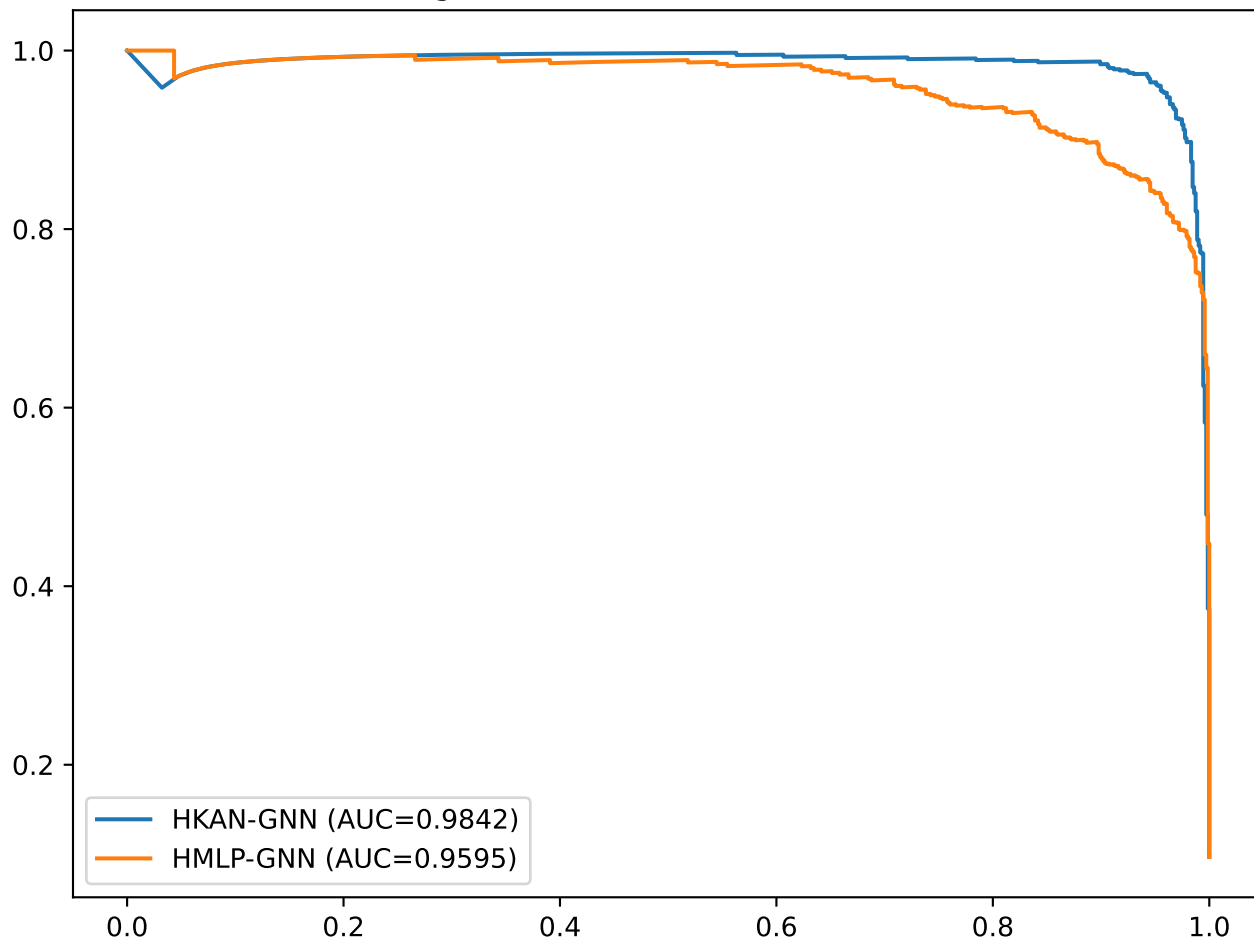
Figure 3: Precision-Recall Curves
