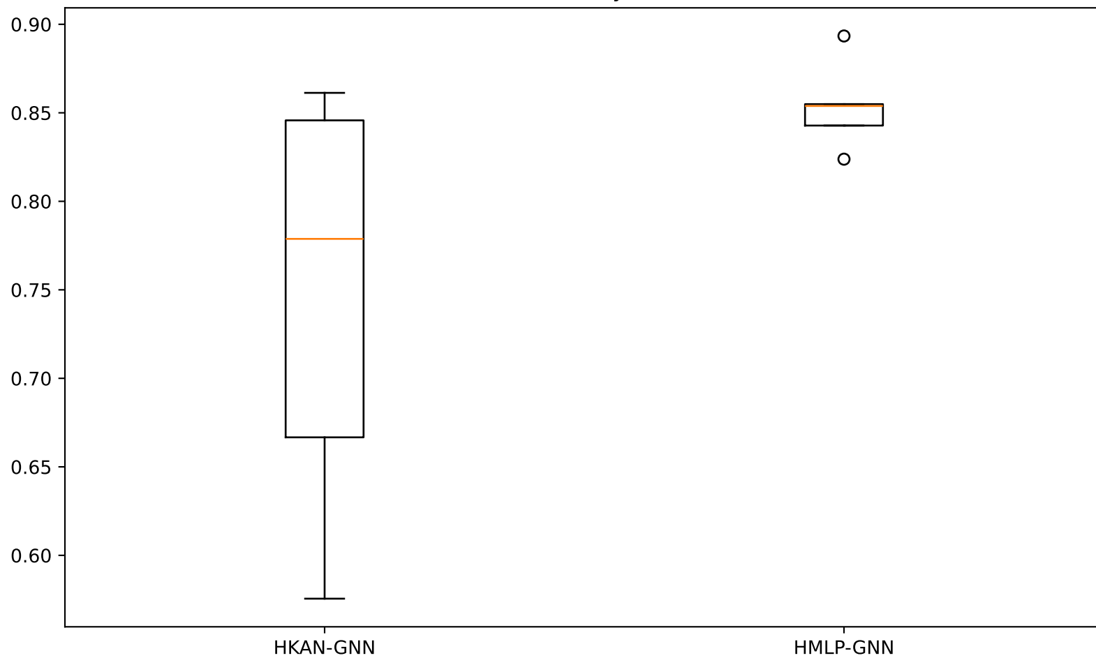
F1-Score Stability (5 Seeds)
