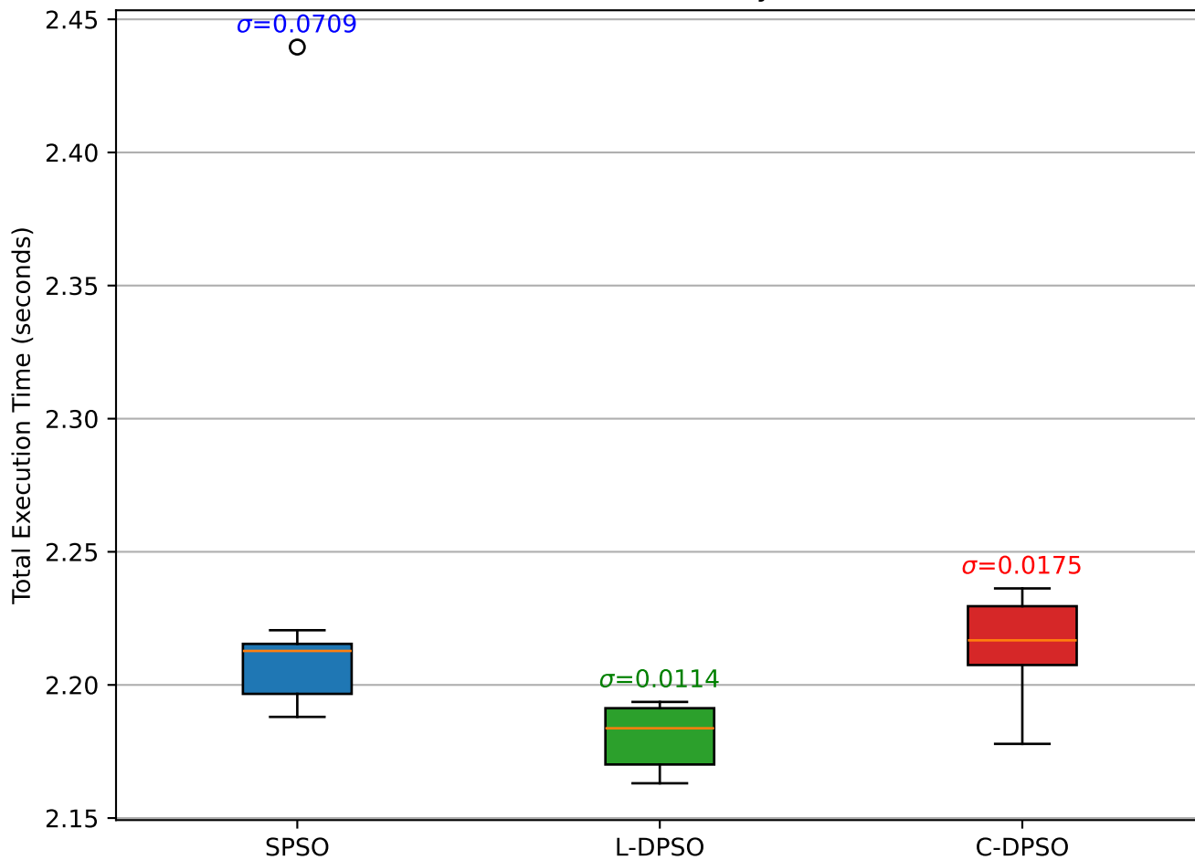
Execution Time Predictability (N=10 Runs)
