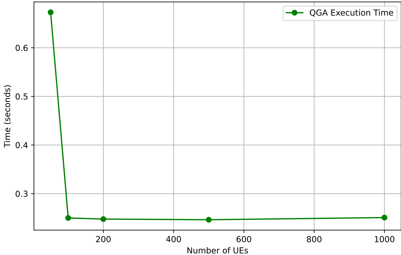
Scalability: Execution Time on RTX 4090
