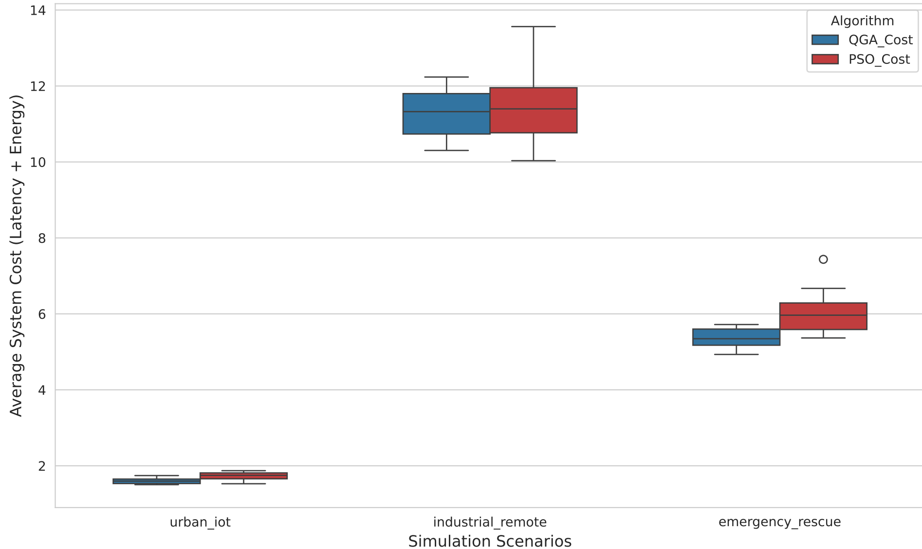
Performance Comparison: Hybrid QGA vs Classical PSO
