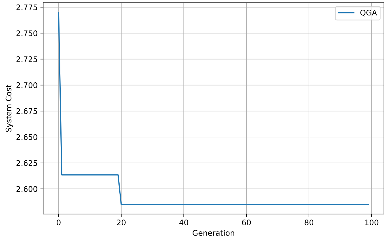
Convergence Analysis on RTX 4090
