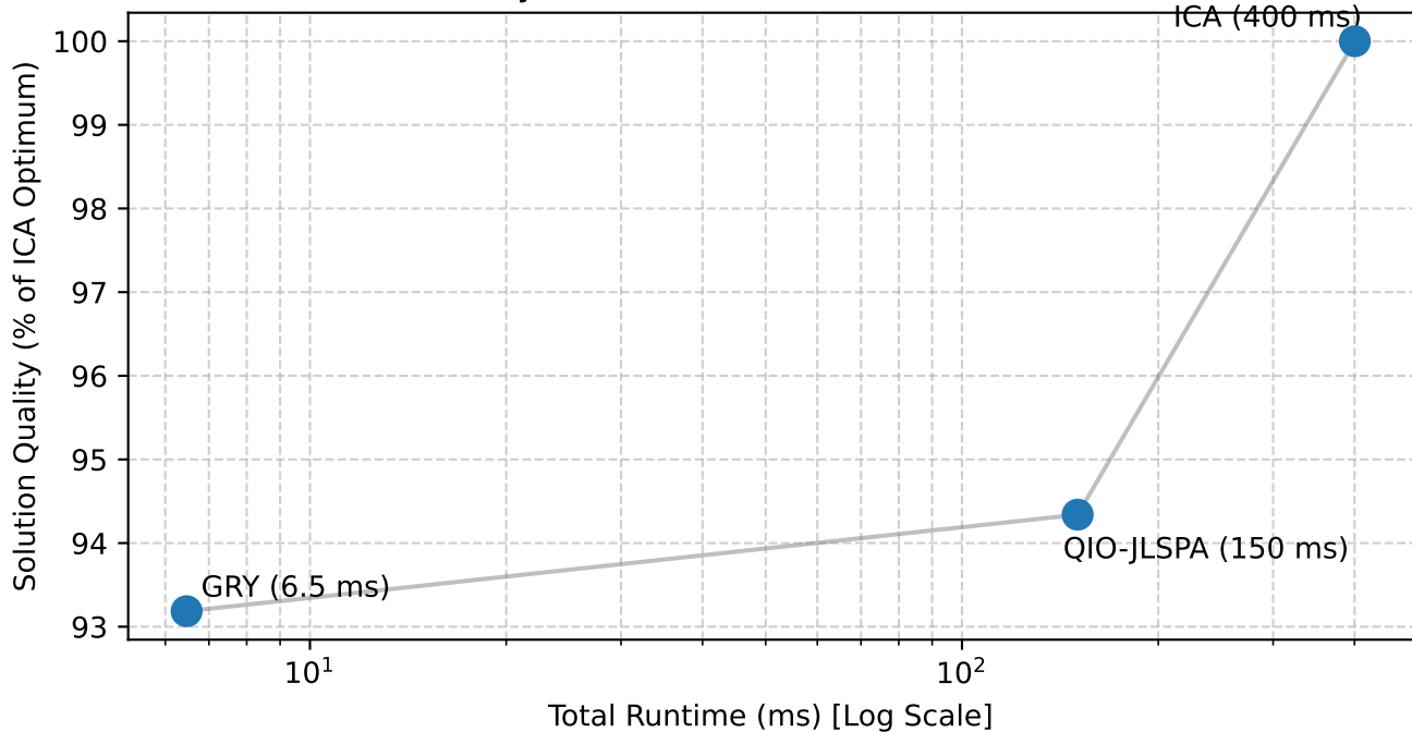
Quality vs. Runtime Trade-off (20 Qubits)
