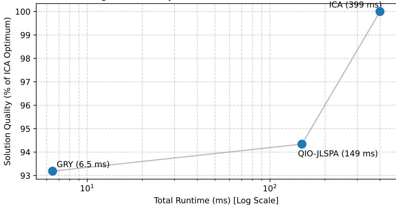
Figure 2: Quality vs. Runtime Trade-off (20 Qubits)
