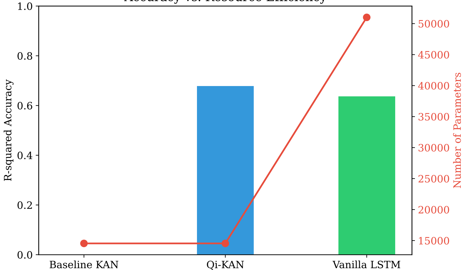
Accuracy vs. Resource Efficiency
