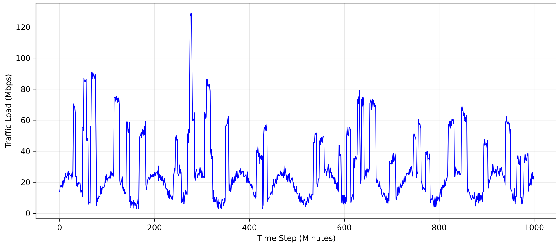
LEO Satellite Traffic Simulation (First 1000 steps)
