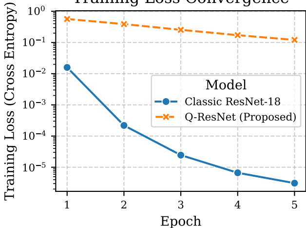
Training Loss Convergence
