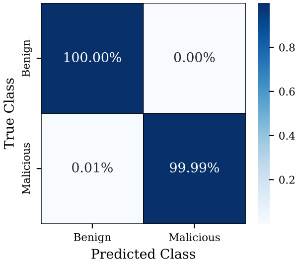
Q-ResNet Confusion Matrix (Normalized)
