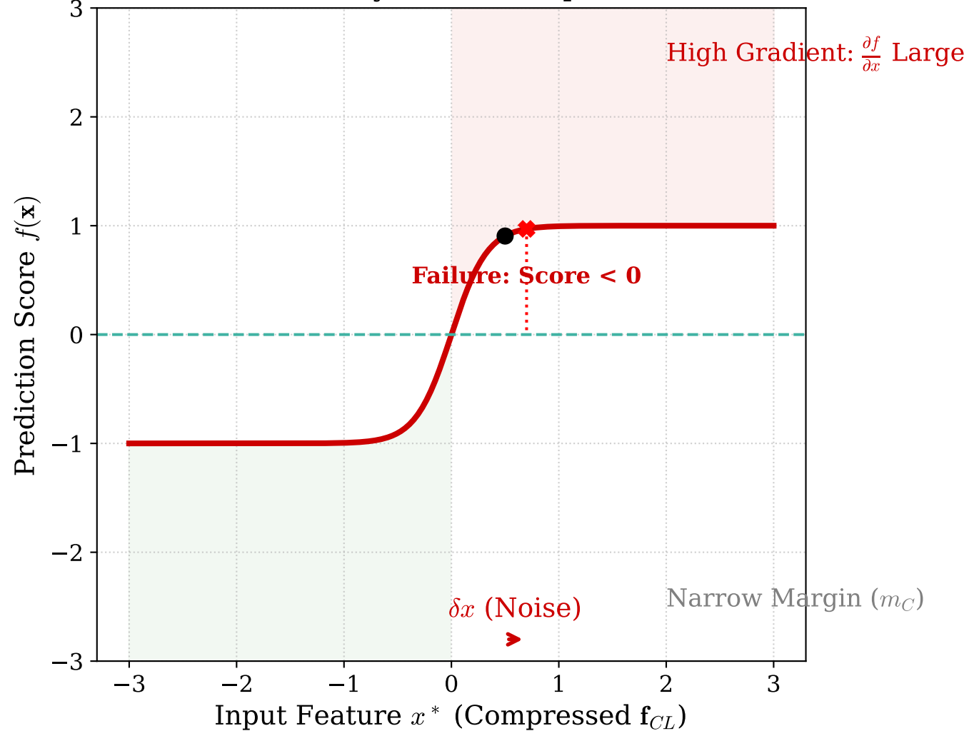
(a) Classical Linear Layer: Catastrophic Failure ( \sigma = 0.4 )
