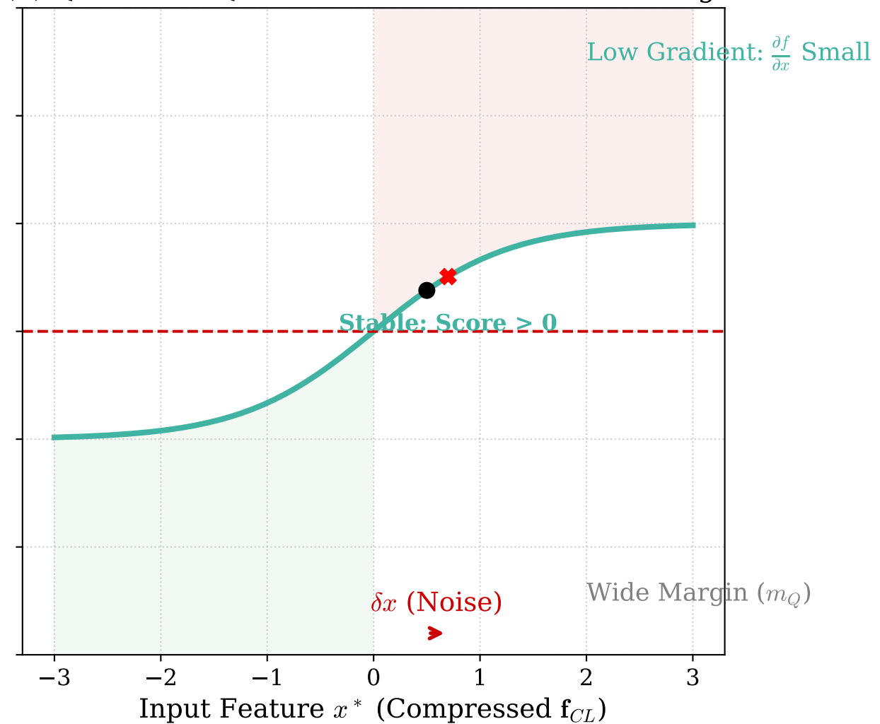
(b) Quantum VQC Kernel: Wide Robustness Margin
