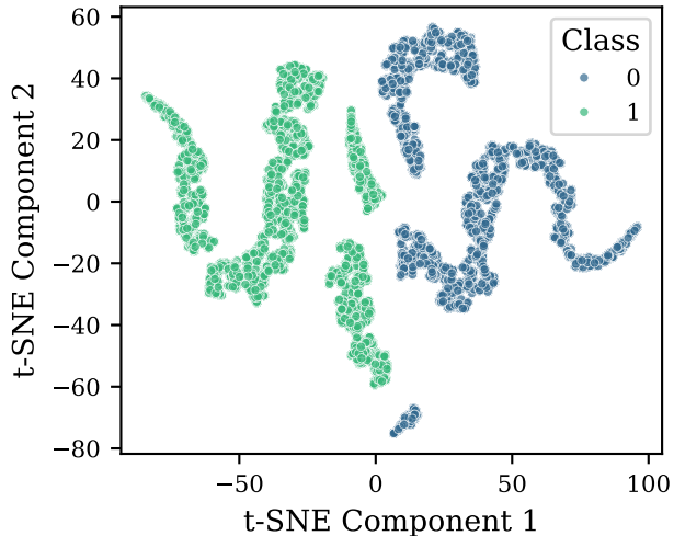
(a) Classic ResNet Feature Space (512D)
