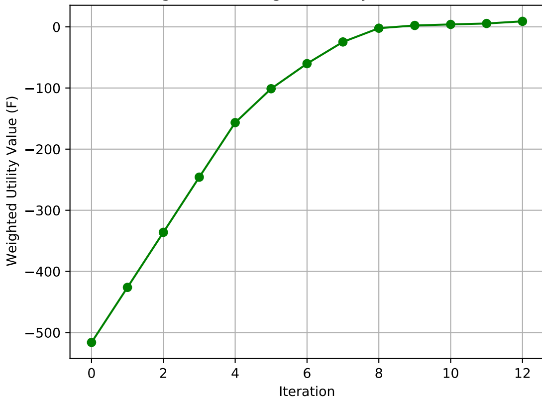
SCA Convergence for Weighted Utility Maximization (Task 3)
