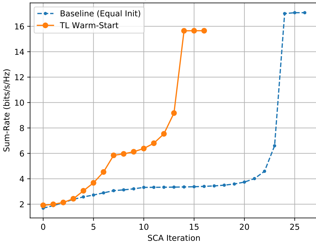
Transfer Learning for SCA Warm-Start (Task 9)
