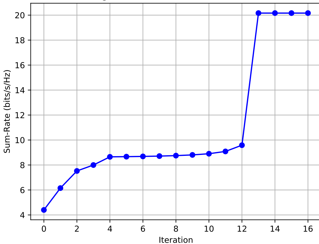
SCA Convergence for Sum-Rate Maximization (Task 1)
