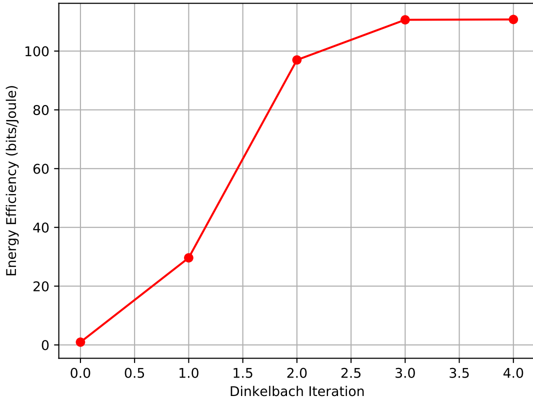
Dinkelbach-SCA Convergence for Energy Efficiency (Task 2)
