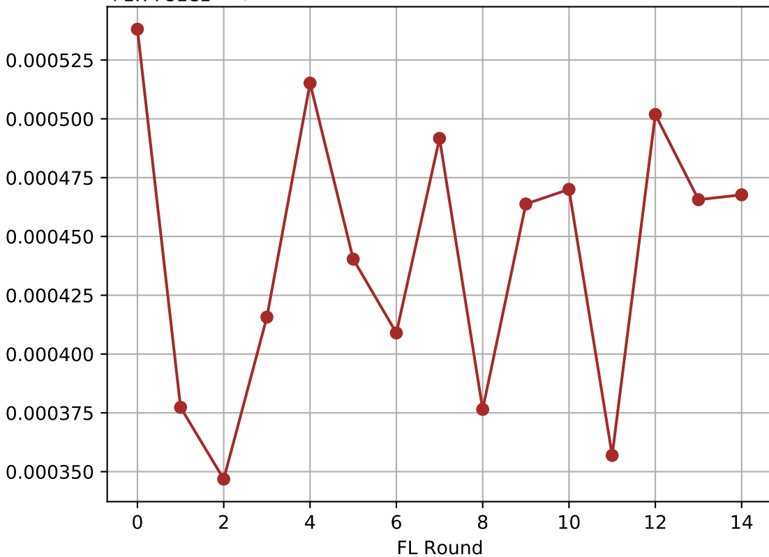
SCA-Optimized FL Communication Rate (Task 7)
