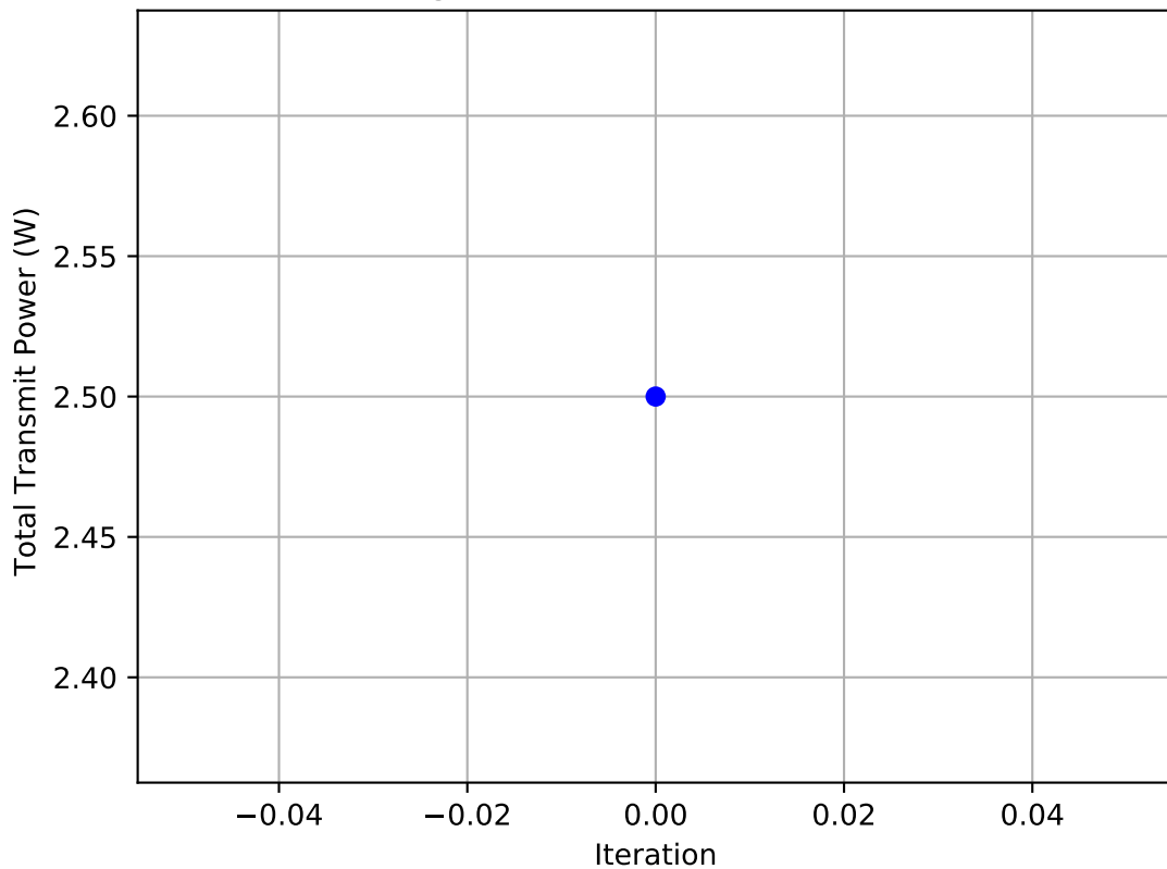
SCA Convergence for Power Minimization (Task 5)
