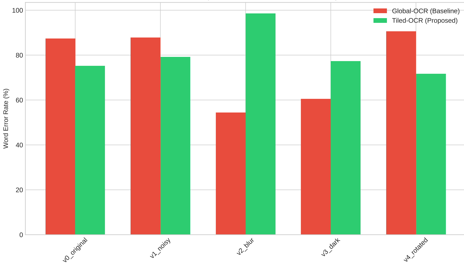
Performance Comparison: Global vs Tiled OCR Strategies
