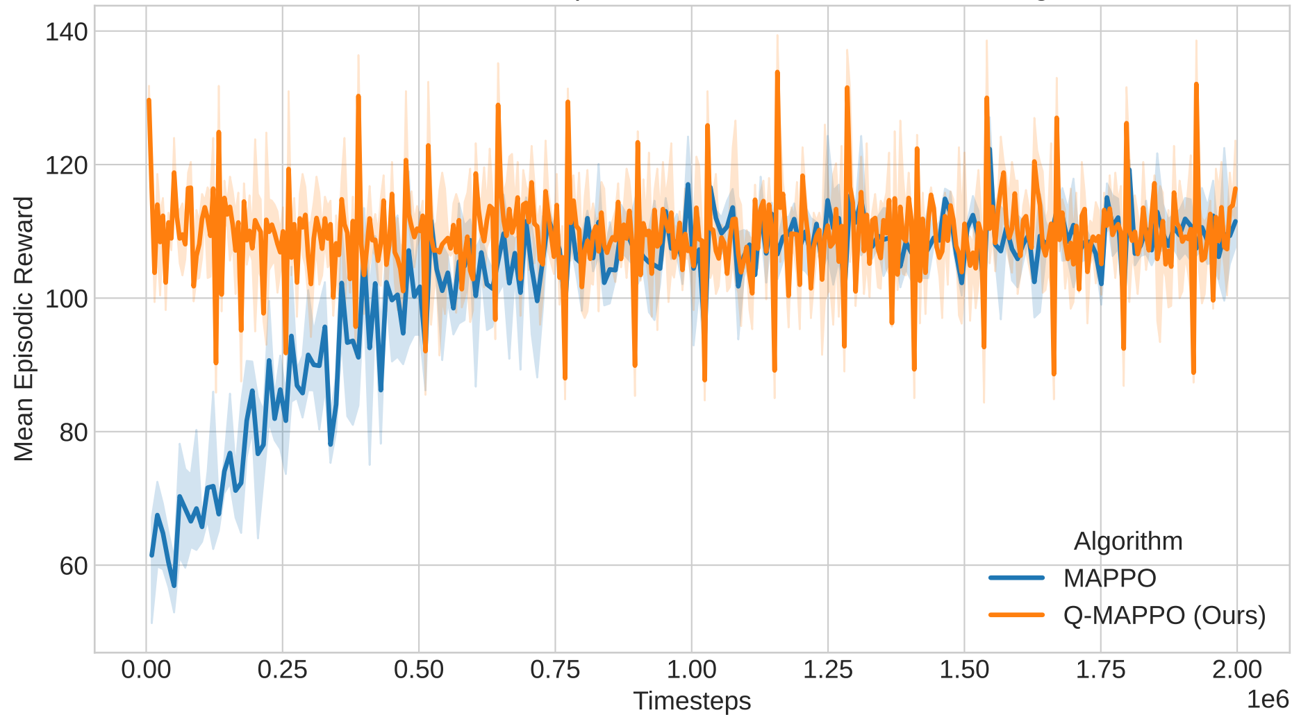
Performance Comparison on Satellite Task Scheduling
