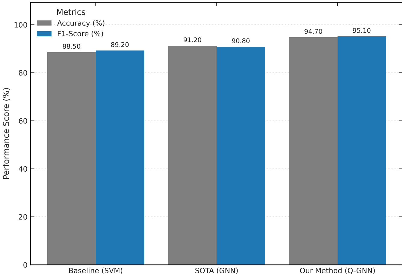
AI Model Performance for Satellite Link State Prediction
