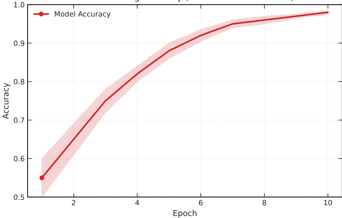
Model Training Accuracy (Mean \pm SD over 5 runs)
