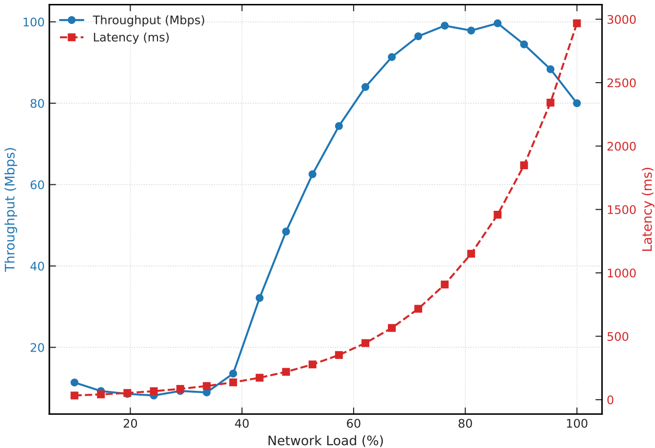
Network Throughput vs. Latency Trade-off
