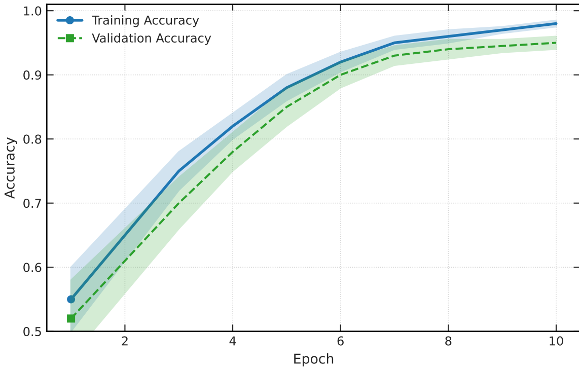
Model Training and Validation Accuracy
