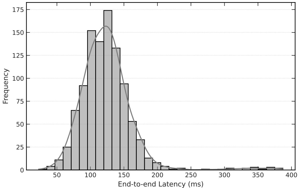
Latency Distribution (Baseline Algorithm)
