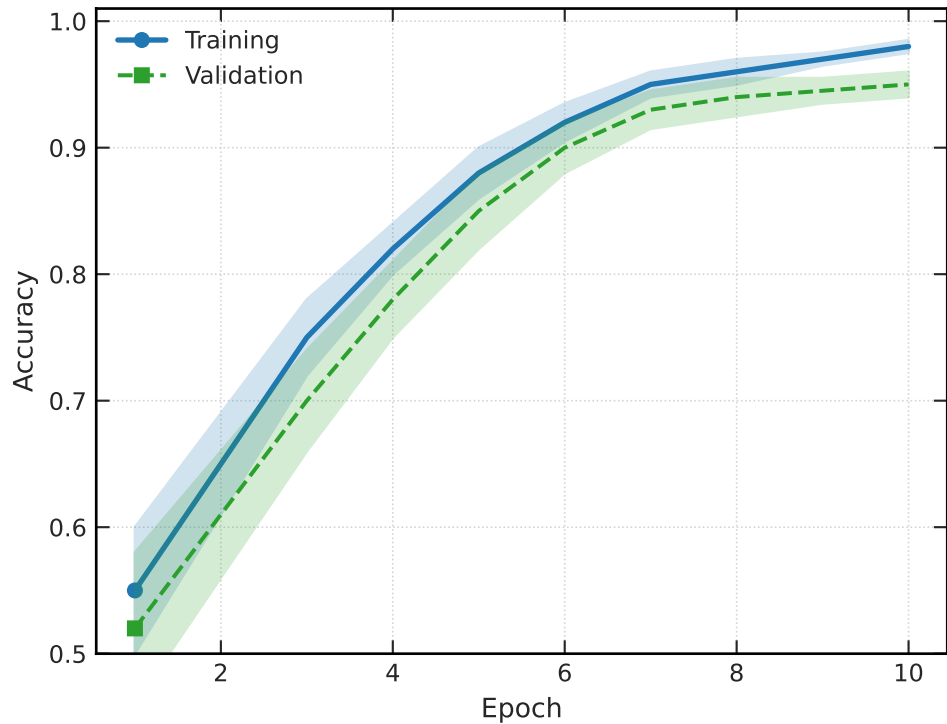
(a) Model Accuracy
