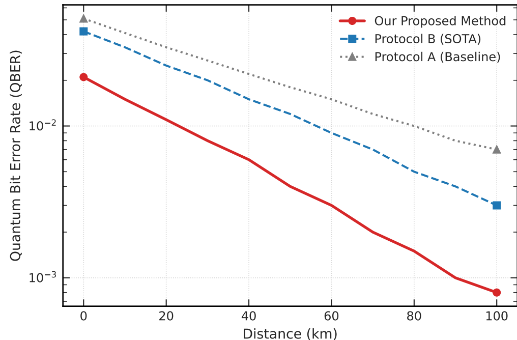
Performance of QKD Protocols (Log Scale)
