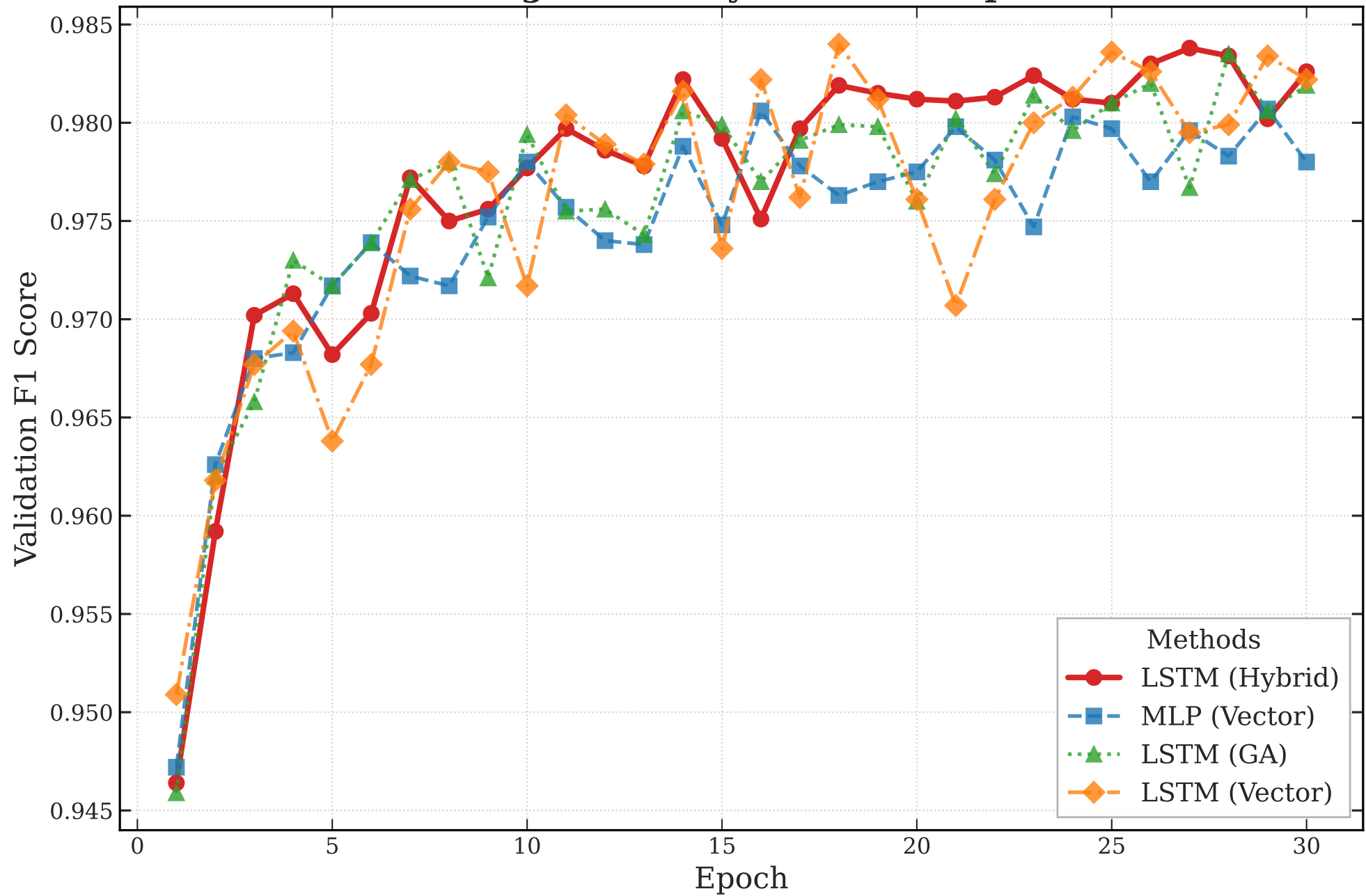
Convergence Analysis over 30 Epochs
