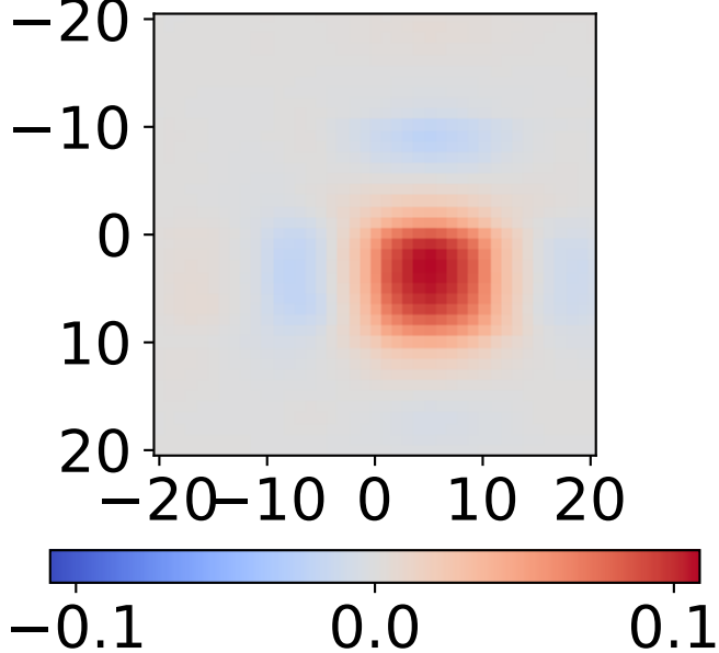
Macroscale kernel 1
