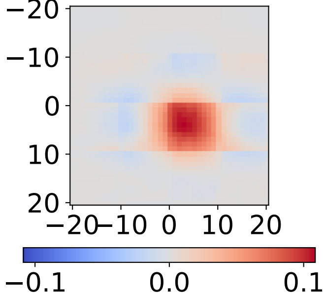
Macroscale kernel 0
