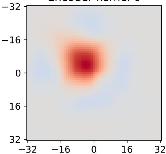
Encoder kernel 0
