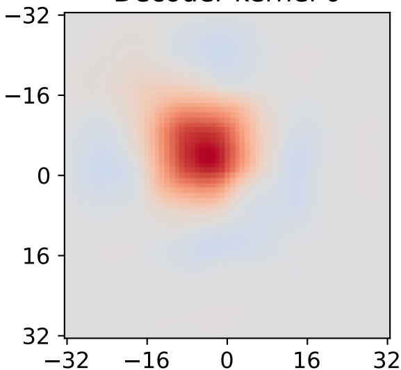
Decoder kernel 0
