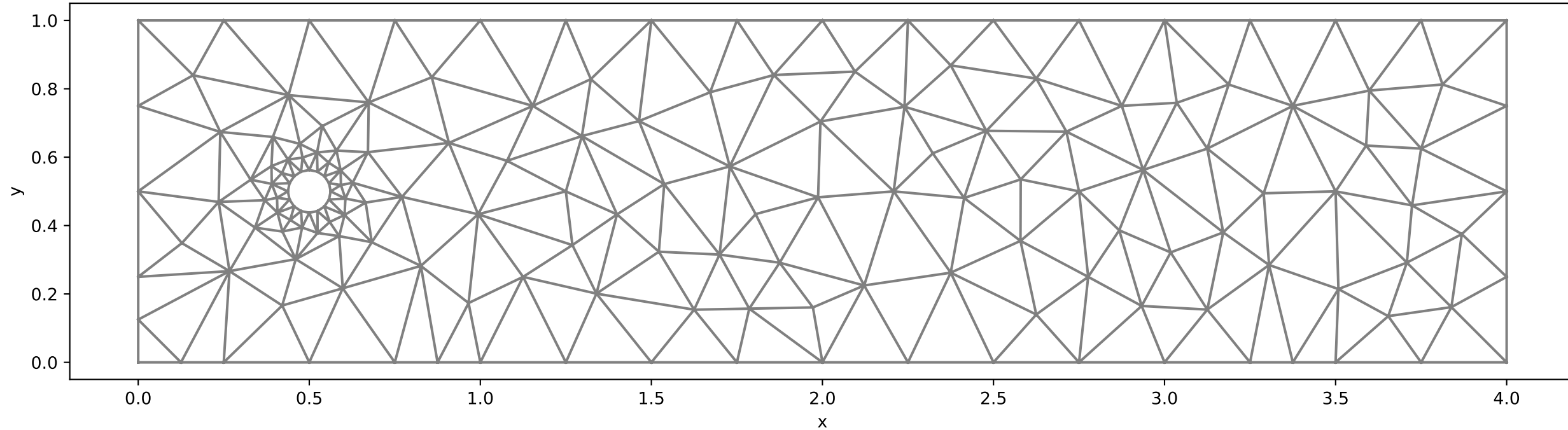
Generated Mesh
