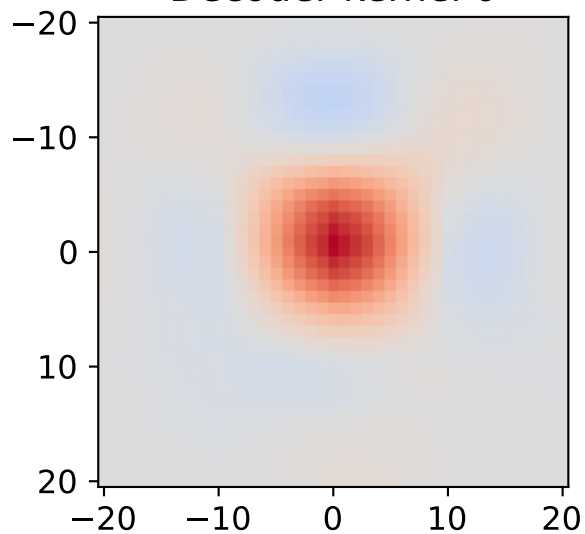
Decoder kernel 0
