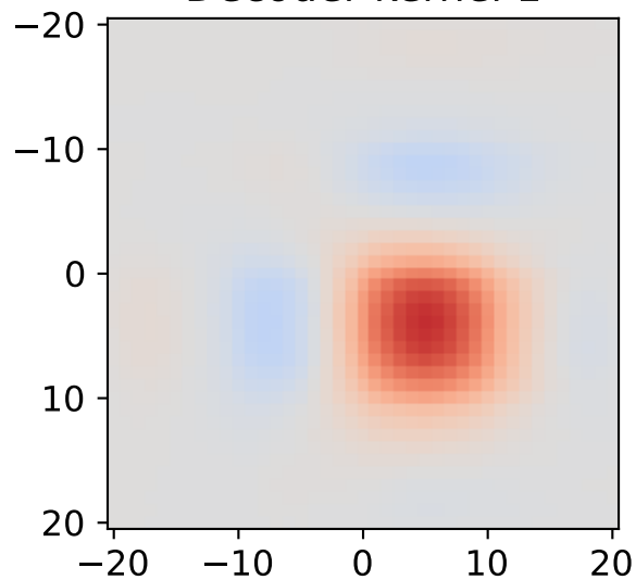
Decoder kernel 1
