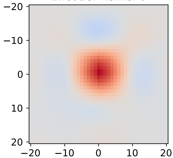
Encoder kernel 0
