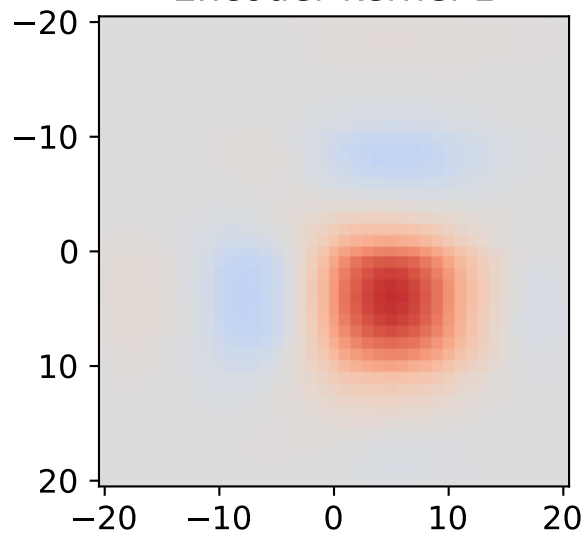
Encoder kernel 1
