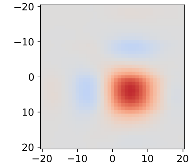
Decoder kernel 1
