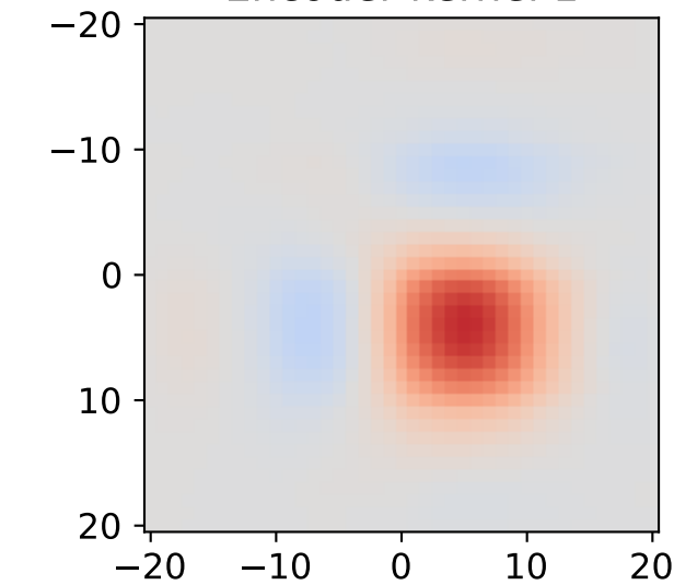
Encoder kernel 1
