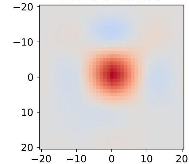
Encoder kernel 0
