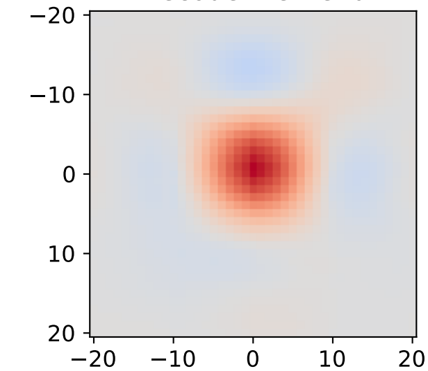
Decoder kernel 0
