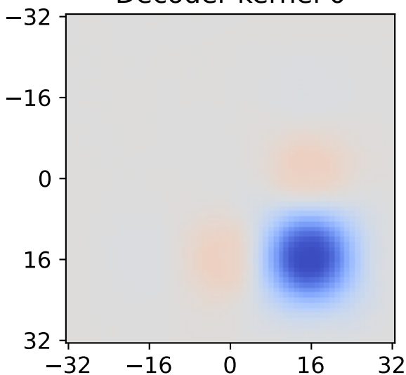
Decoder kernel 0
