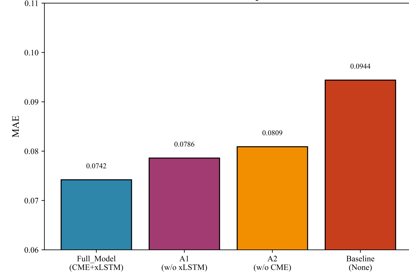
MOSI: MAE Comparison
