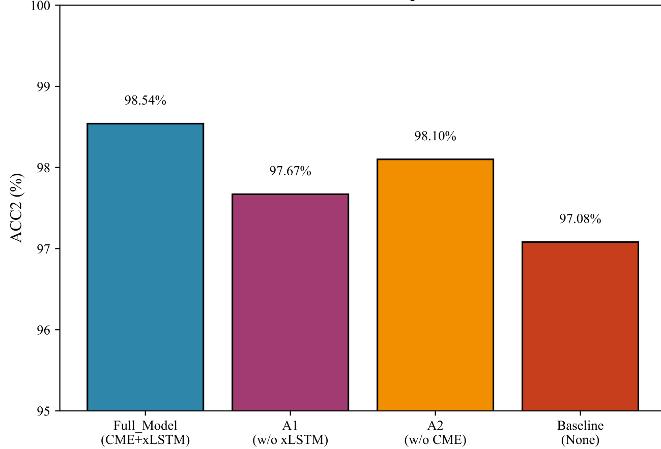
MOSI: ACC2 Comparison
