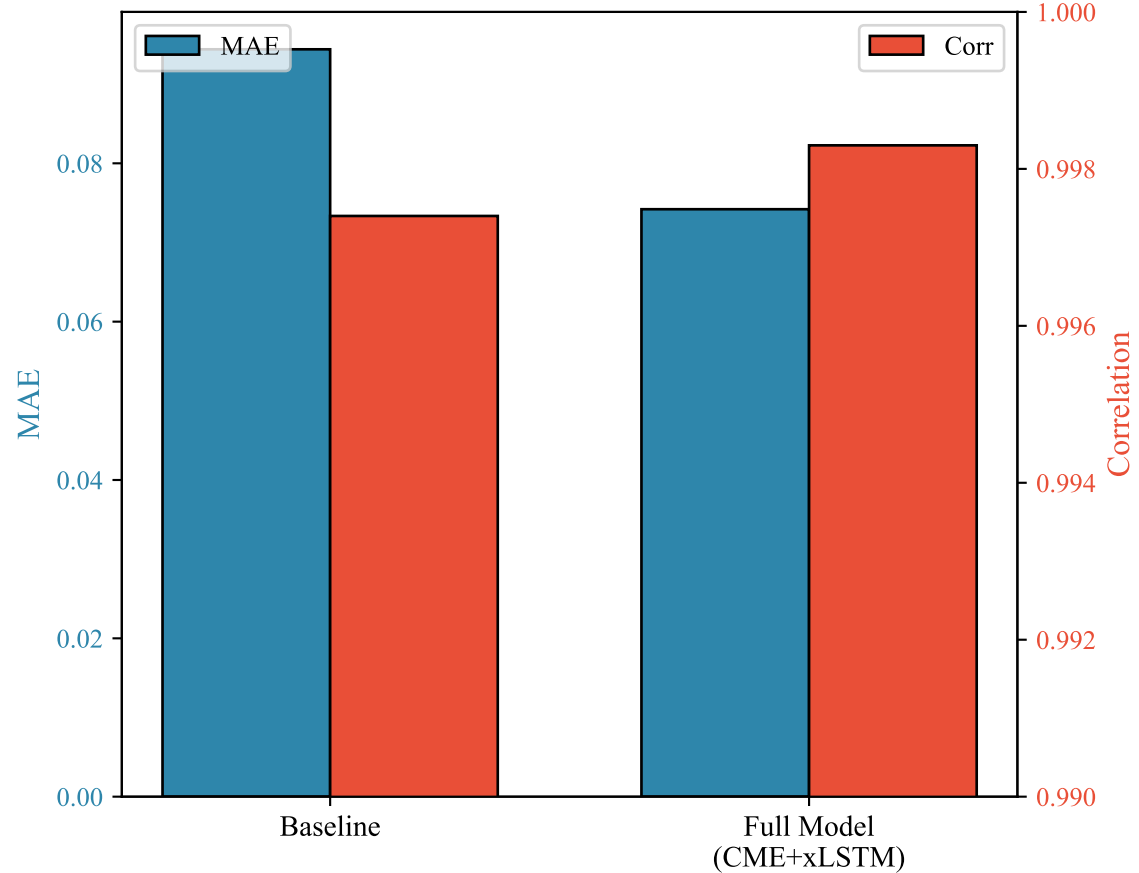
MOSI: xLSTM Contribution
