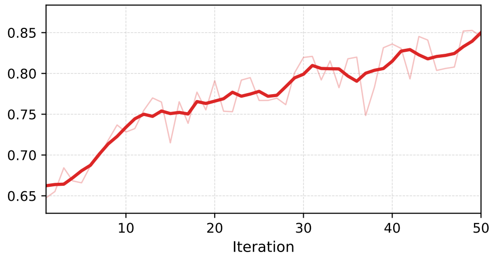
Command resilience
