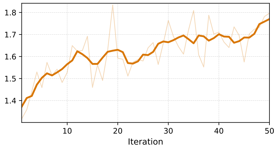
Command resilience
