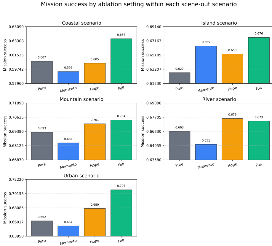
Figure 3: Mission success by ablation setting within each of the five scene-out scenarios in the canonical generalization suite. Each panel uses a locally tightened y-axis range to make between-group differences easier to inspect. The plotted values come from the corresponding best_simulation.mission_success fields in the per-scene full_result.json files.
