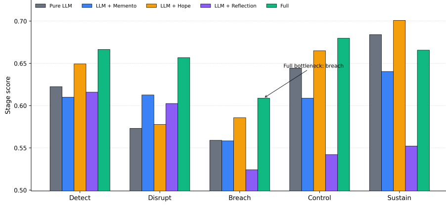
Figure 2: Five-stage kill-chain scores for the canonical single-scenario ablation (RTX 4090 D). The figure visualizes the same values reported in Table 5. The Full pipeline leads four of the five stages (detect, disrupt, breach, control); in the sustain stage the Hope-only variant retains the highest bar. breach remains the weakest Full-stage score and therefore the most explicit residual bottleneck.
