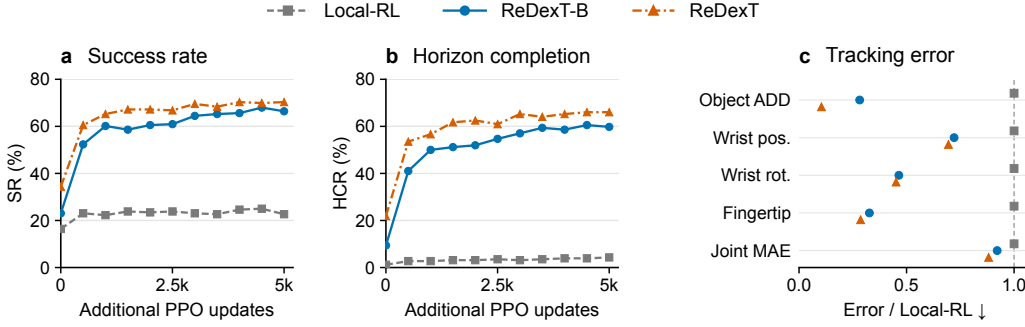
Figure 4: Adaptation to 256 new trajectories from random, bootstrap, and expanded initializations. (a,b) Success and horizon completion over 5,000 PPO updates. (c) Final object and hand errors on 55 common successes, normalized by Local-RL for each metric; lower is better.
