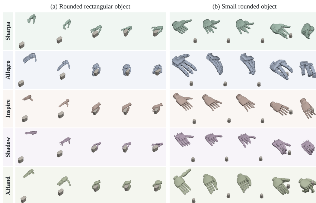
Figure 8: Frozen-policy rollouts across hands with (a) a rounded rectangular object and (b) a small rounded object.
