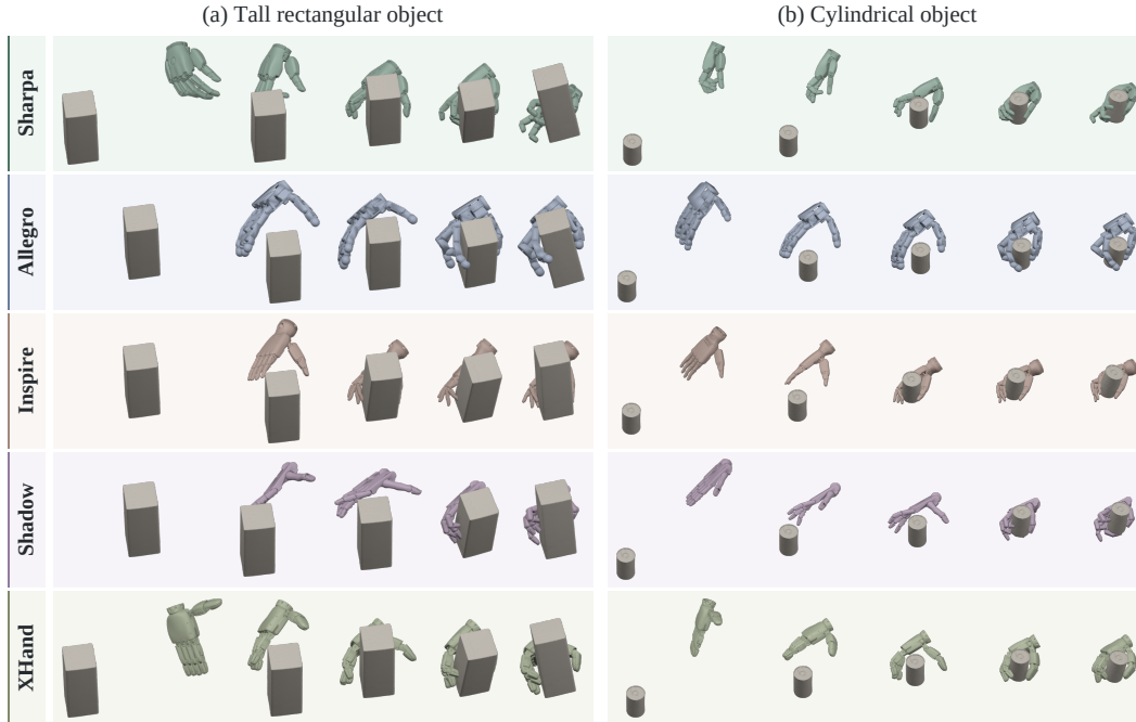
Figure 7: Frozen-policy rollouts across hands with (a) tall rectangular and (b) cylindrical objects.
