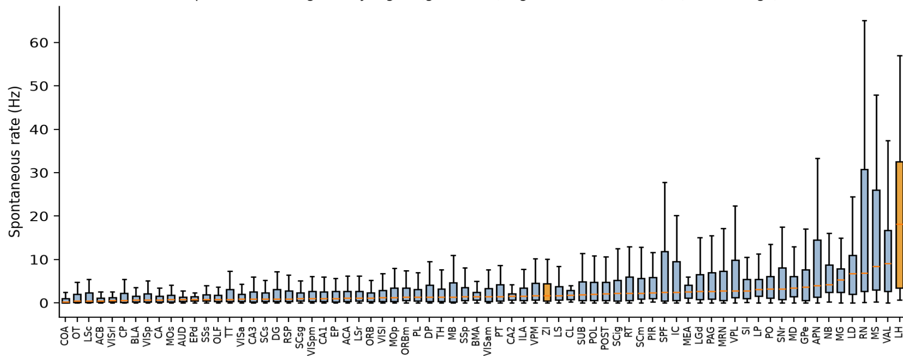
Spontaneous firing rate by region (good units; regions with \geq 20 units; ZI/LH in orange)
