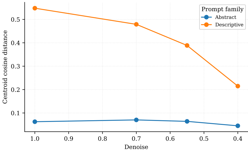
Distance to Unconditioned centroid by denoise
