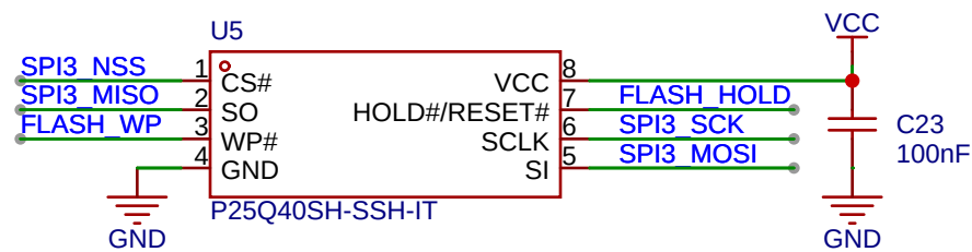
NOR FLASH
