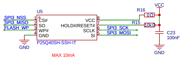
NOR FLASH
