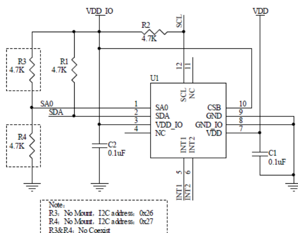
Figure 12 da217E I2C electrical connect
