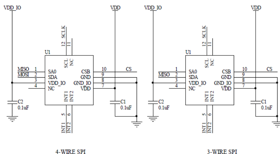
Figure 13 da217E SPI electrical connect
