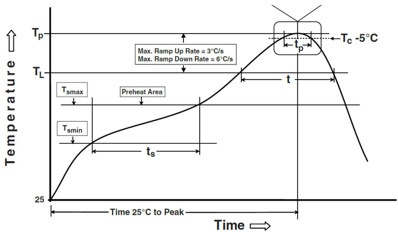
Figure 16 Soldering profile
