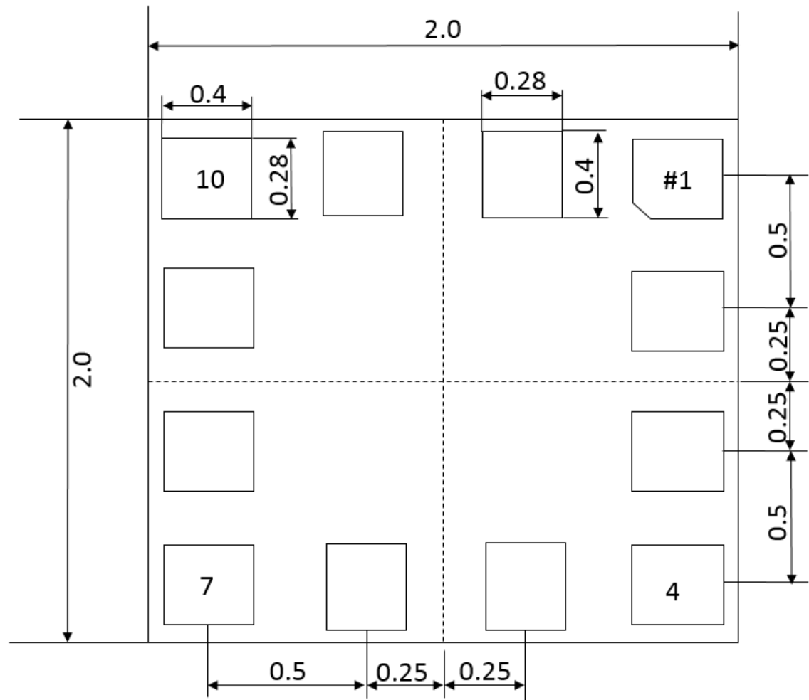
Bottom View
