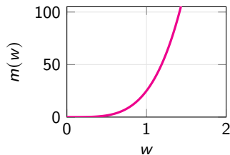
Polynomial: 25w^4
