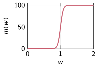
Sharp logistic: a = 25
