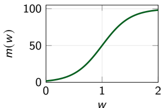
Smooth logistic: a = 4
