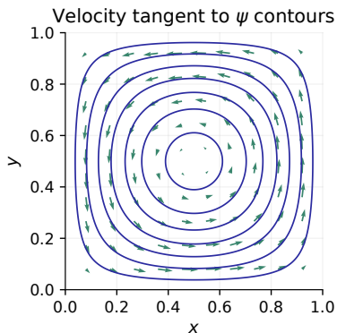
Exact illustration: \psi = \sin(\pi x) \sin(\pi y) .
