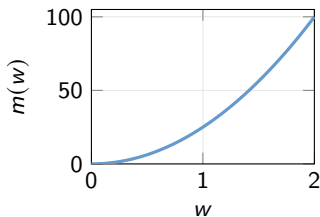
Polynomial: 25w^2
