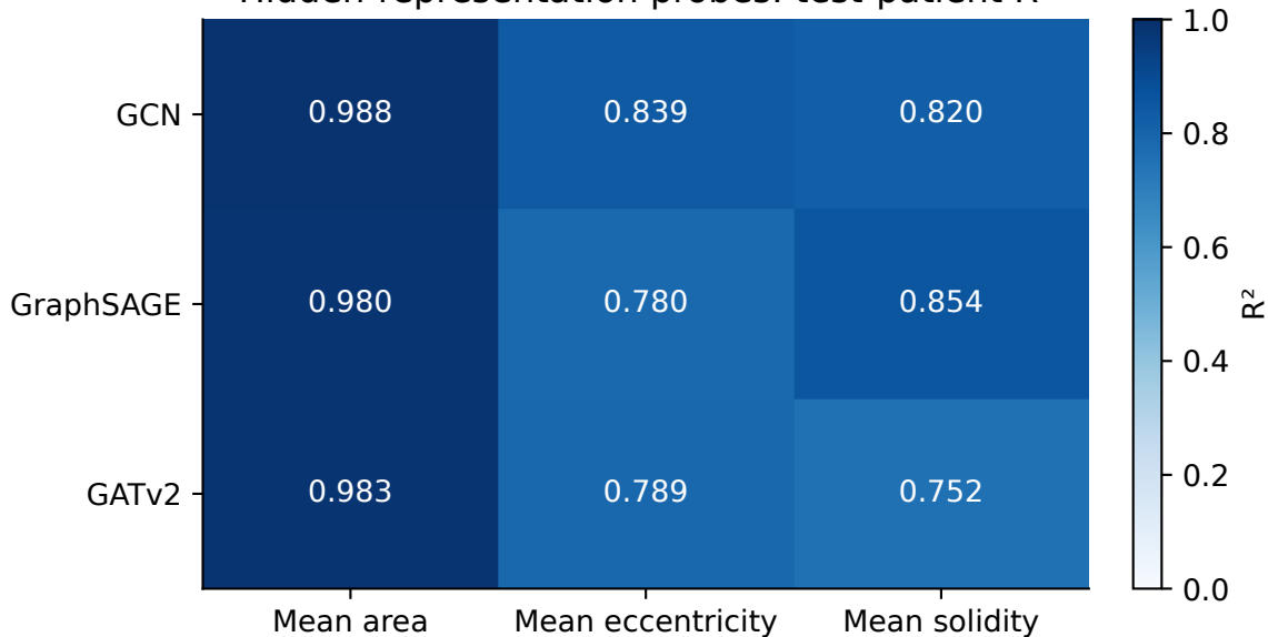
Hidden-representation probes: test-patient R^2
