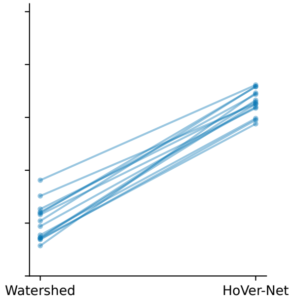
Panoptic quality
