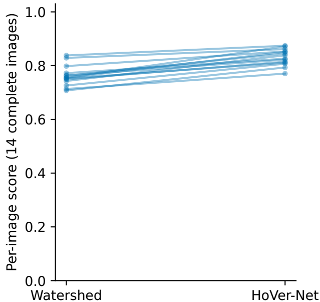
Foreground Dice
