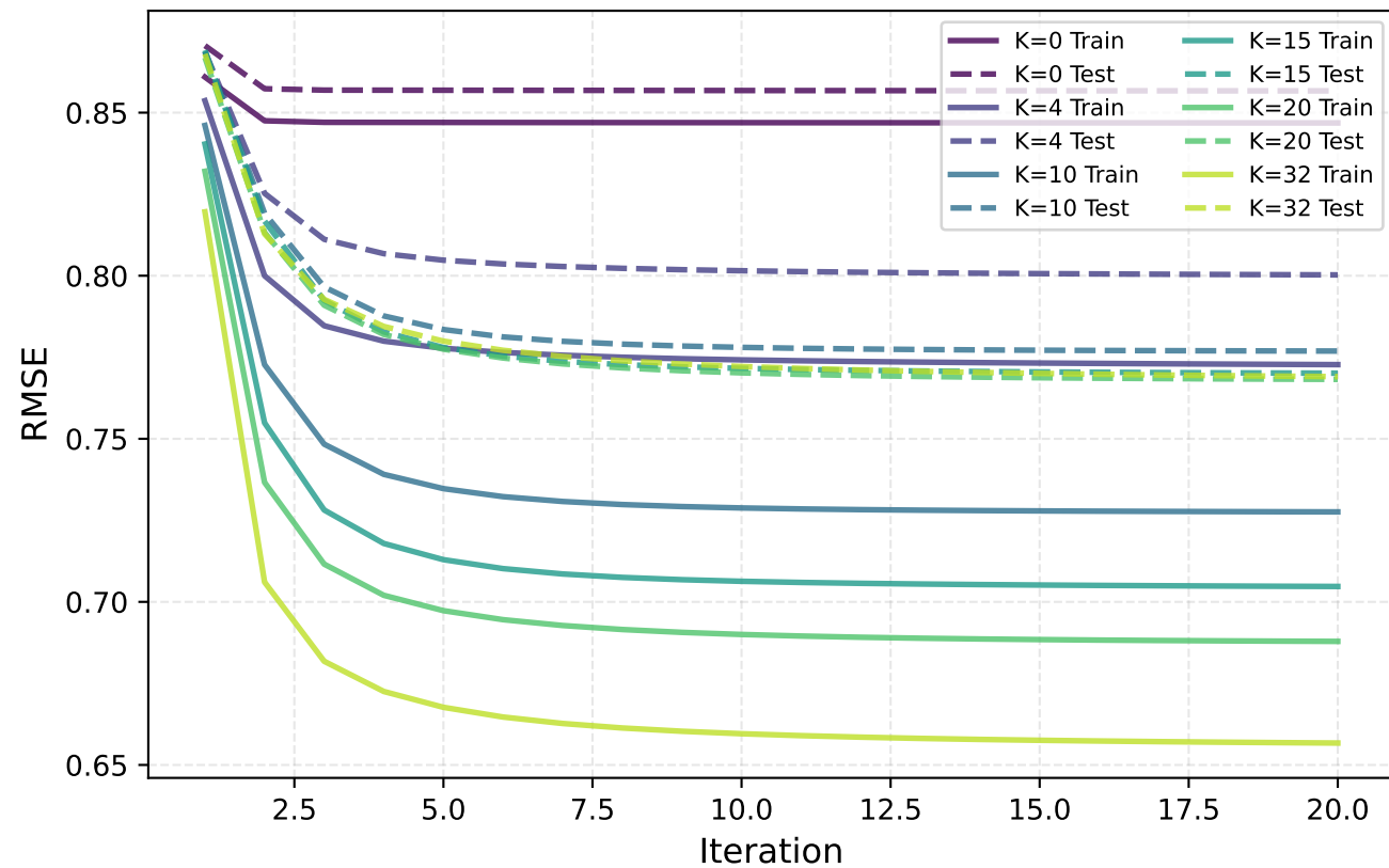
Train/Test RMSE Evolution (gap shows overfitting)
