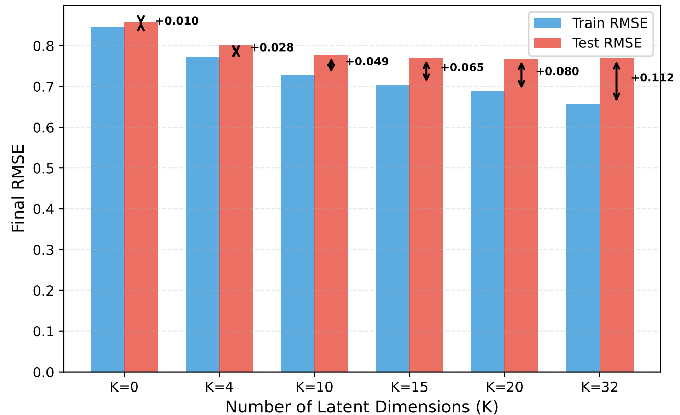
Final RMSE vs K (arrow = overfitting gap)
