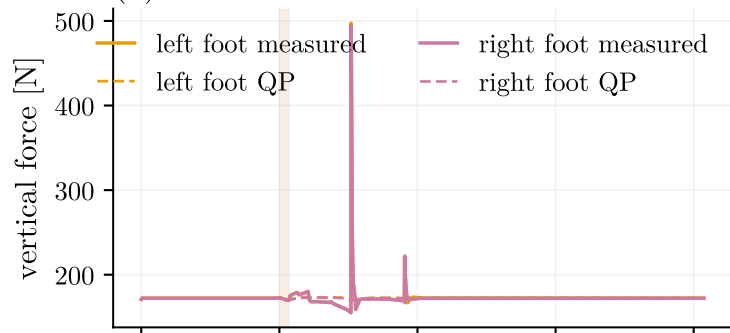
(a) vertical GRF
