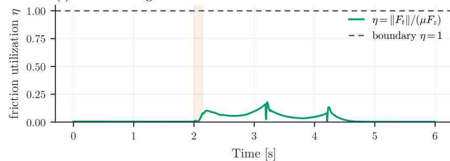
(f) friction margin
